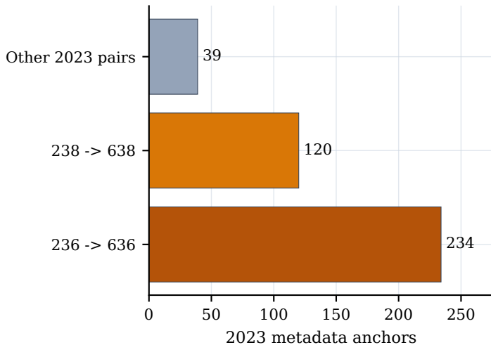
Named code-pair concentration
