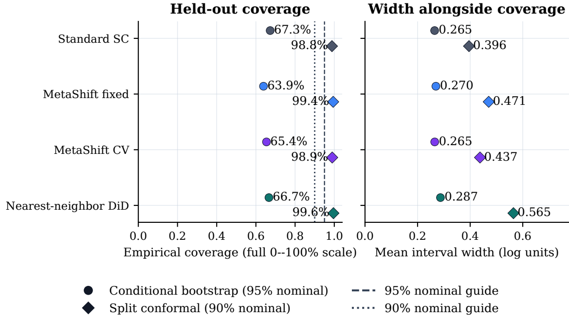
Figure 8: Held-out synthetic interval coverage and mean width. Fixed conditional intervals under-cover their nominal 95% target, whereas split-conformal intervals over-cover their nominal 90% target. The figure reports a calibration limitation, not a real-event confidence guarantee.
