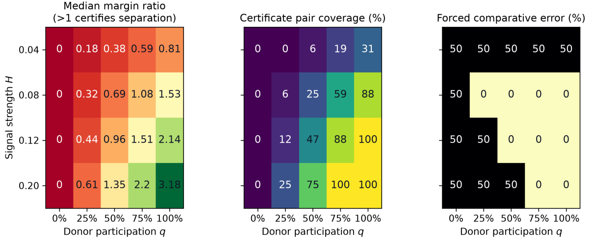
Figure 4: Structural answerability boundary on the held-out grid. From left to right, the panels show the median normalized structural margin, certificate answered-pair coverage, and forced-comparative scope error. Values above one in the first panel meet the sufficient interval-separation condition. Each cell averages over the five adverse comparison factors; q = 0 remains the observational-identity negative control.
