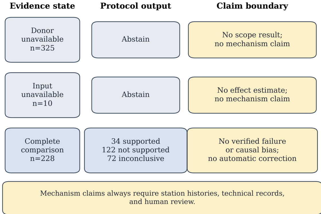
Figure 22: Claim-boundary matrix for the AQS audit. Rows partition all 563 primary anchors into donor-insufficient, input-window-failure, and complete-comparison states; the complete row separately reports observational evidence tiers. Every row excludes a physical-mechanism conclusion.
