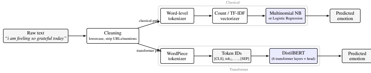
Figure 1. Emotion-classification pipeline. Raw text is cleaned once, then routed through a classical path (word-level tokenizer → count / TF-IDF vectorizer → Naive Bayes or Logistic Regression) or a transformer path (WordPiece tokenizer → integer token IDs → fine-tuned DistilBERT).
