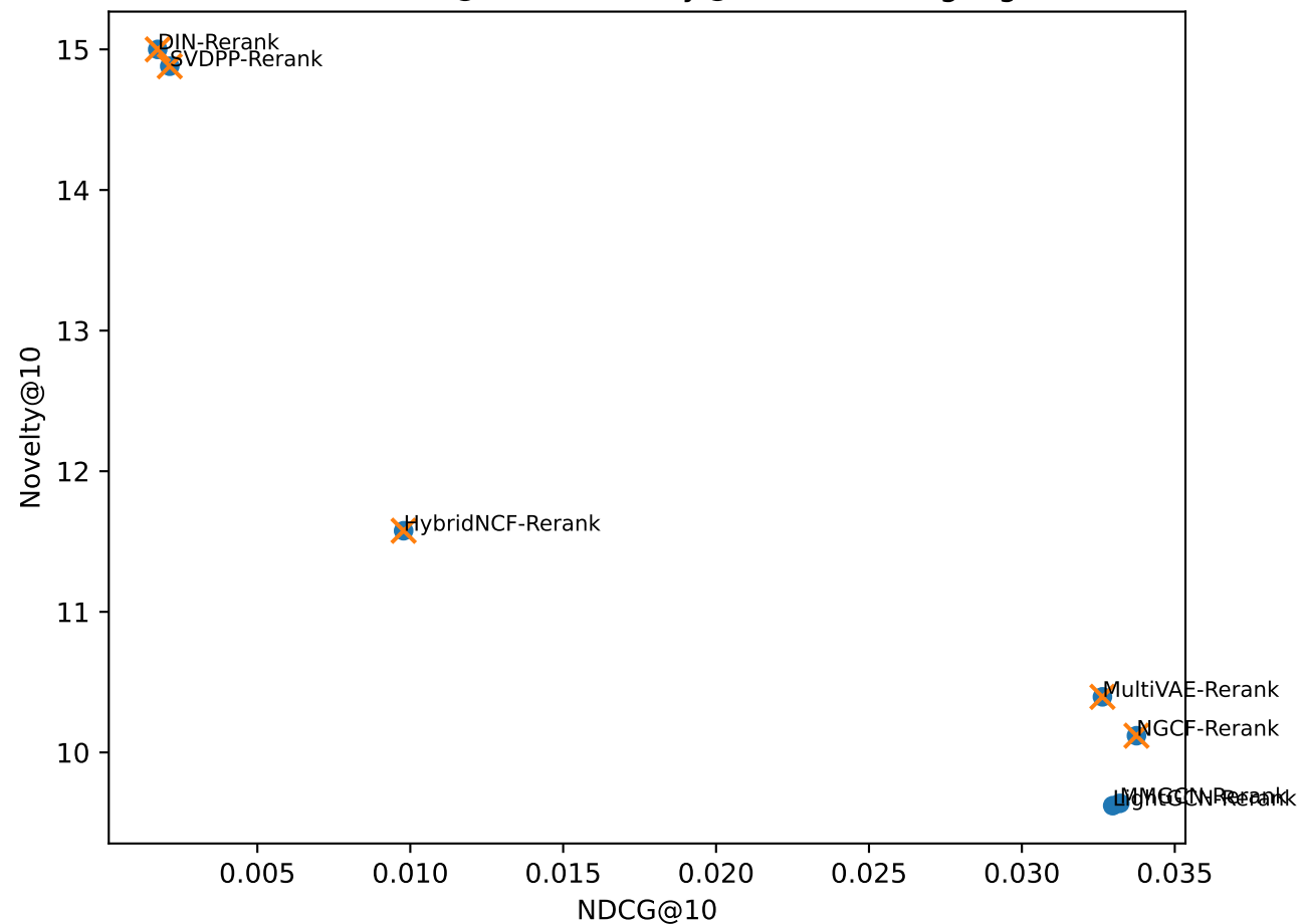
Trade-off: NDCG@10 vs Novelty@10 (Pareto highlighted)
