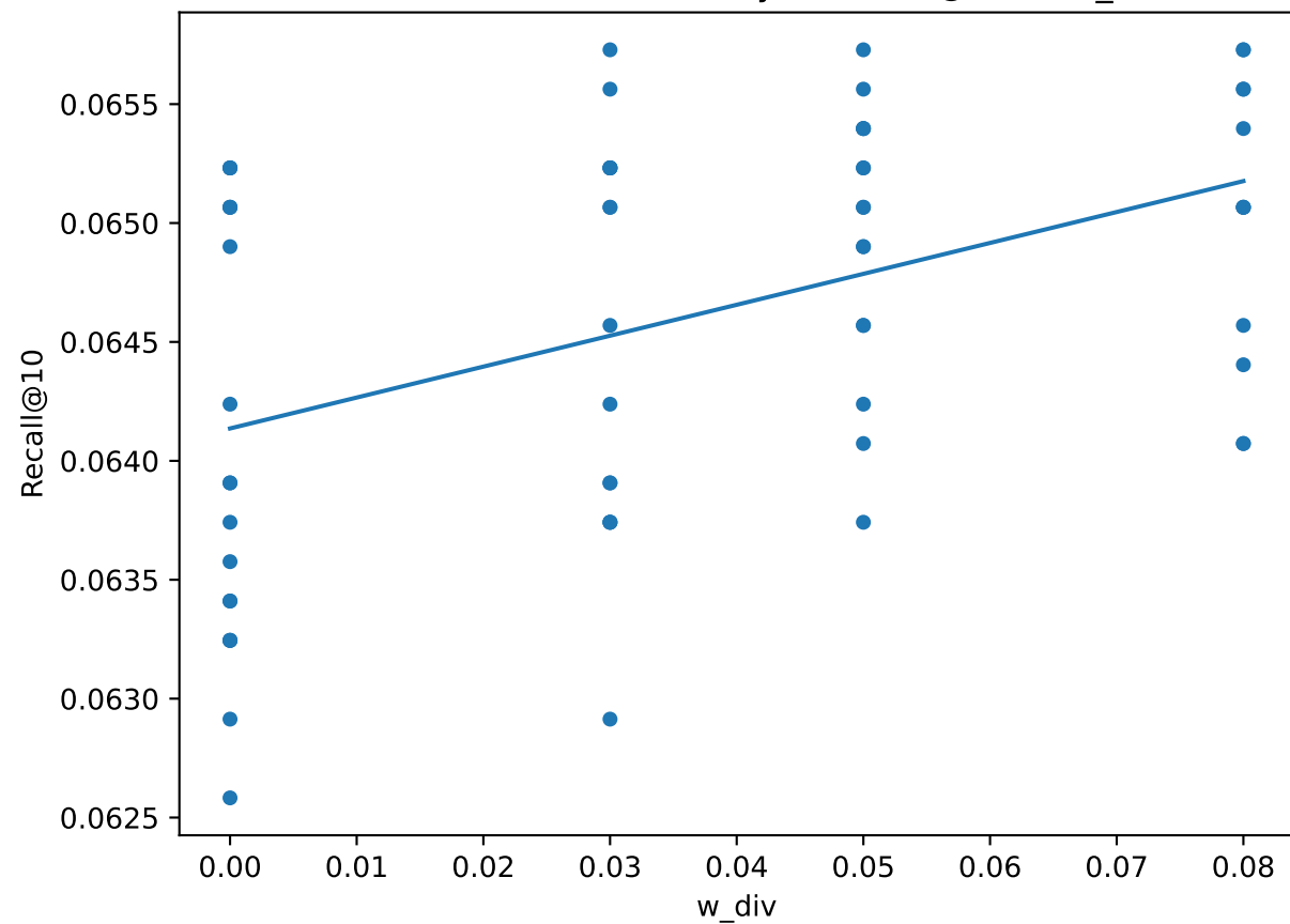
MMGCN-Rerank: Sensitivity of Recall@10 to w_div
