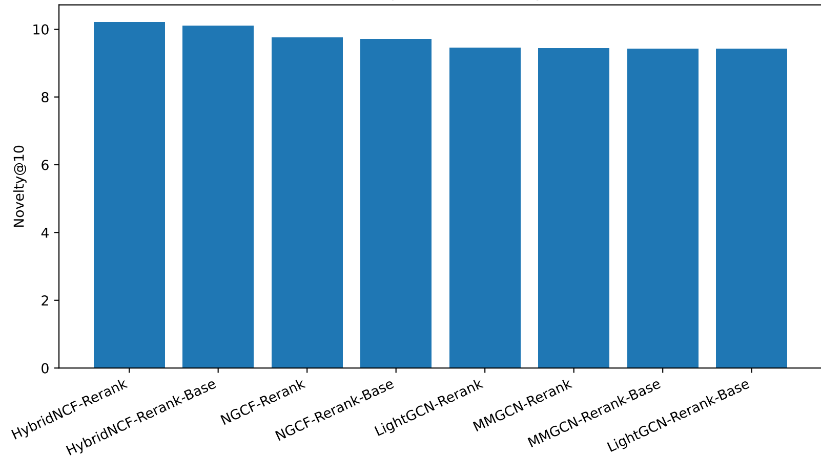
Model Comparison on Novelty@10
