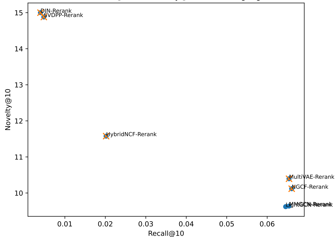
Trade-off: Recall@10 vs Novelty@10 (Pareto highlighted)
