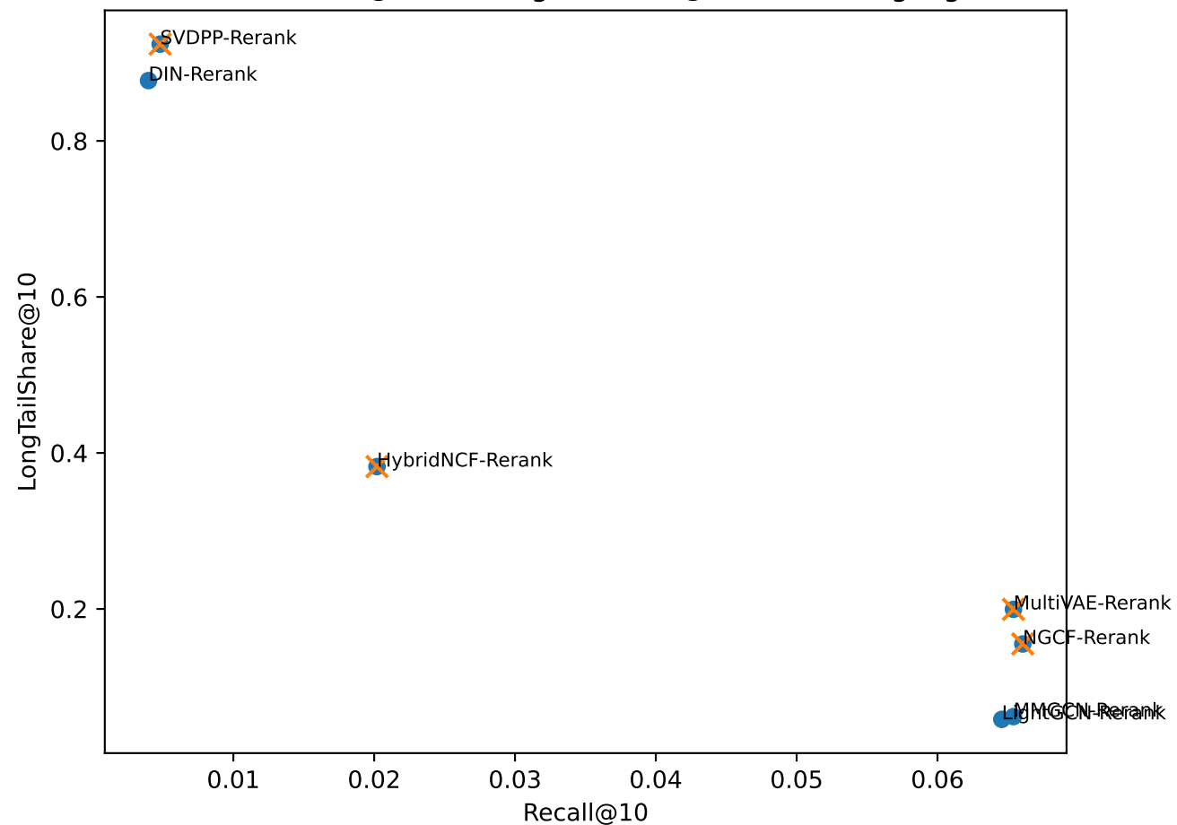
Trade-off: Recall@10 vs LongTailShare@10 (Pareto highlighted)
