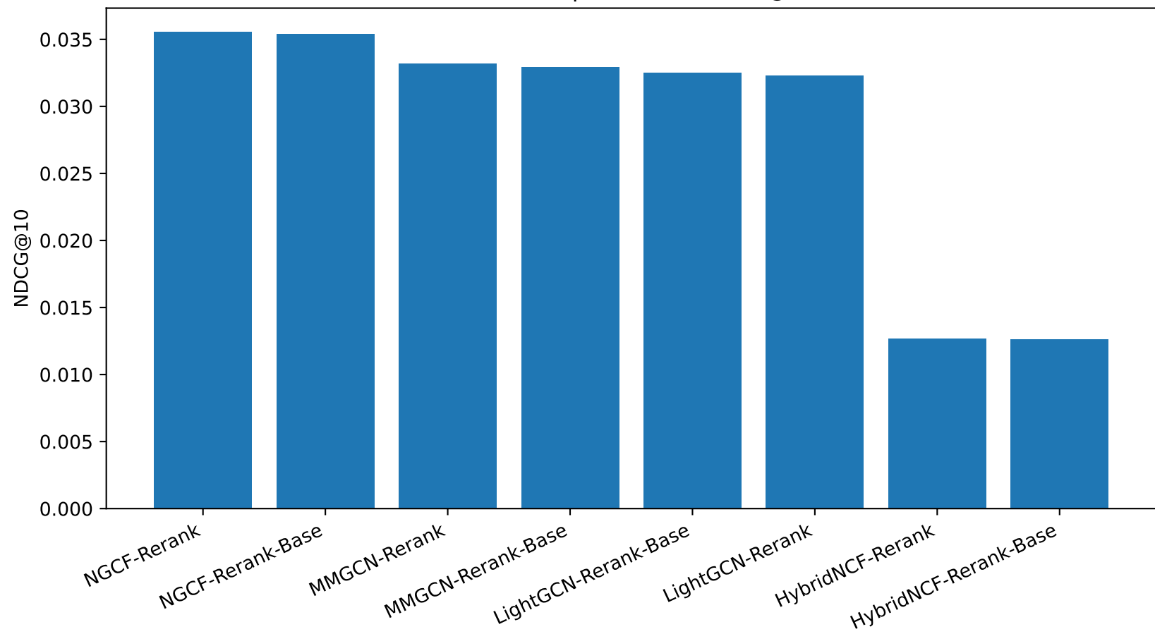
Model Comparison on NDCG@10
