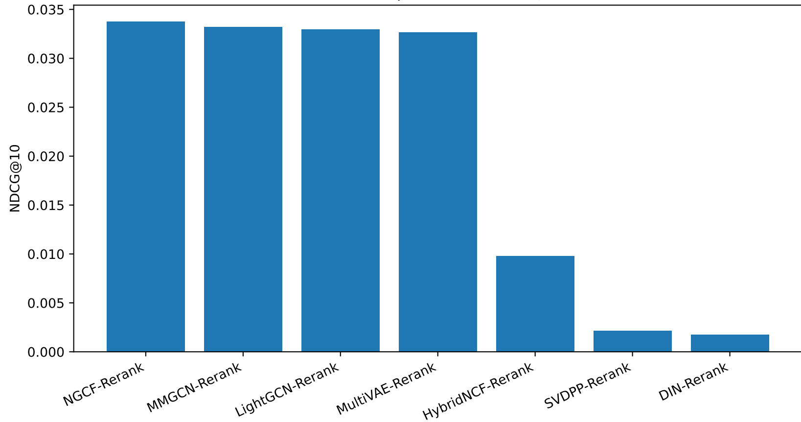
Model Comparison on NDCG@10
