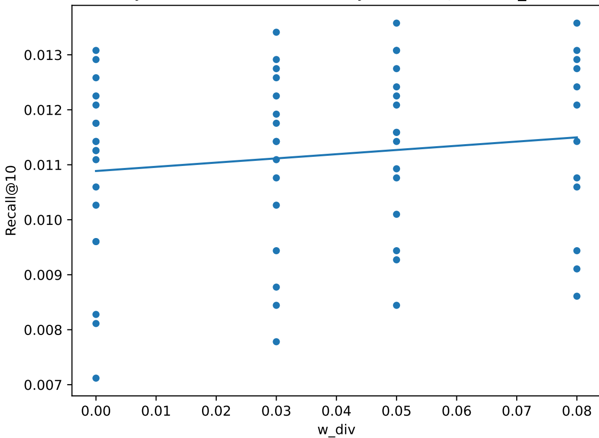
HybridNCF-Rerank: Sensitivity of Recall@10 to w_div
