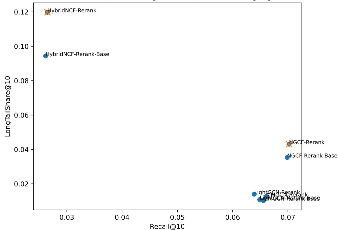
Trade-off: Recall@10 vs LongTailShare@10 (Pareto highlighted)
