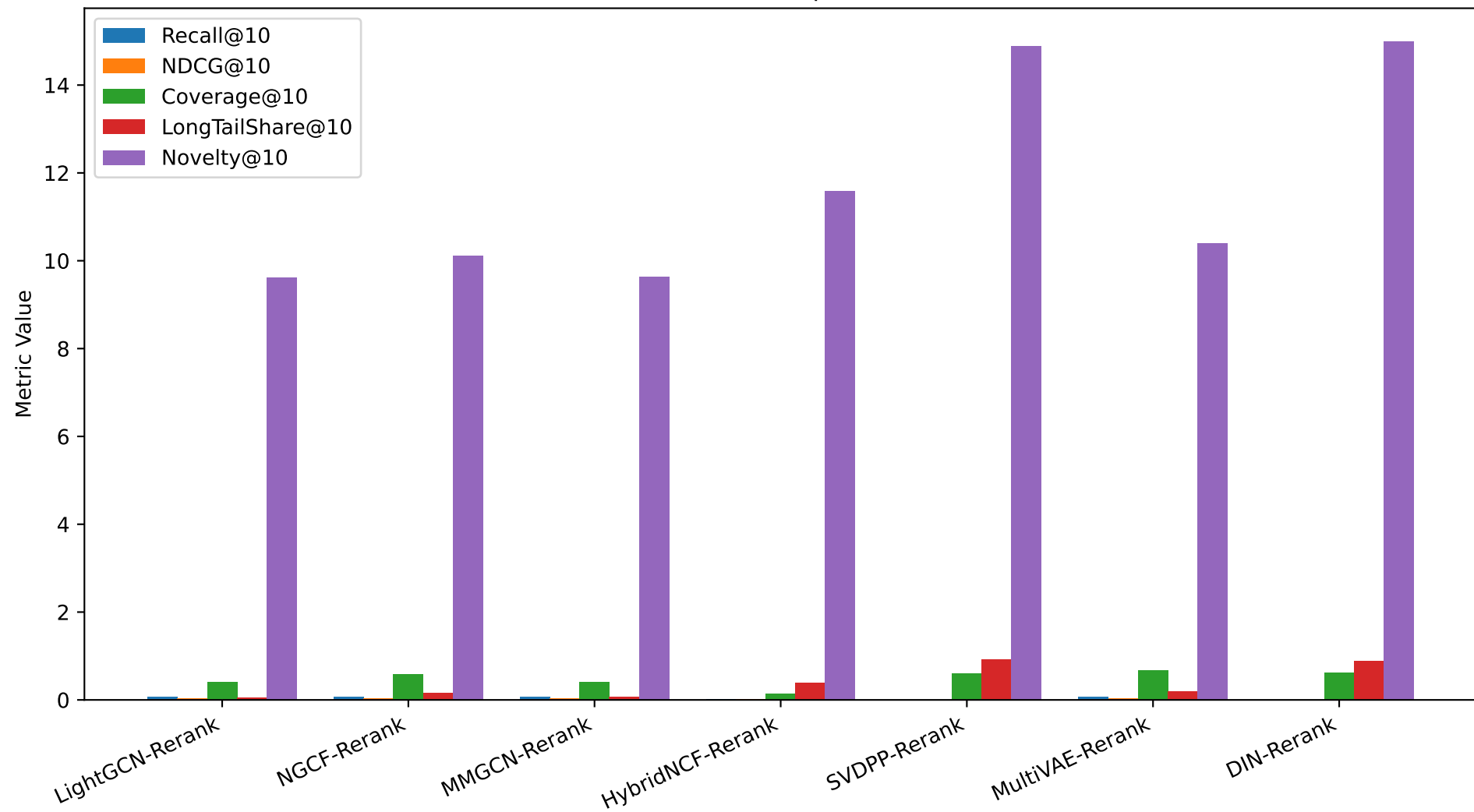
Overall Metrics Comparison (K=10)
