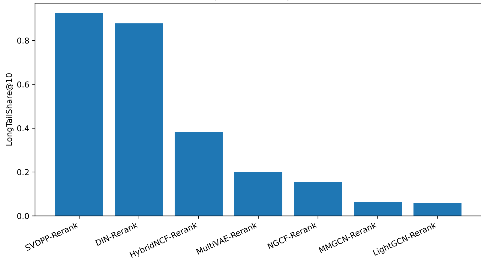
Model Comparison on LongTailShare@10
