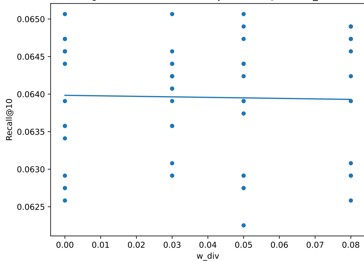
LightGCN-Rerank: Sensitivity of Recall@10 to w_div
