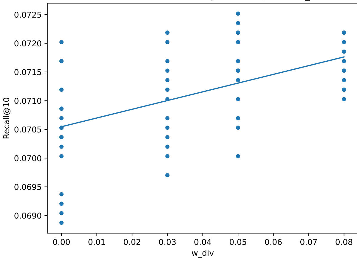
MultiVAE-Rerank: Sensitivity of Recall@10 to w_div
