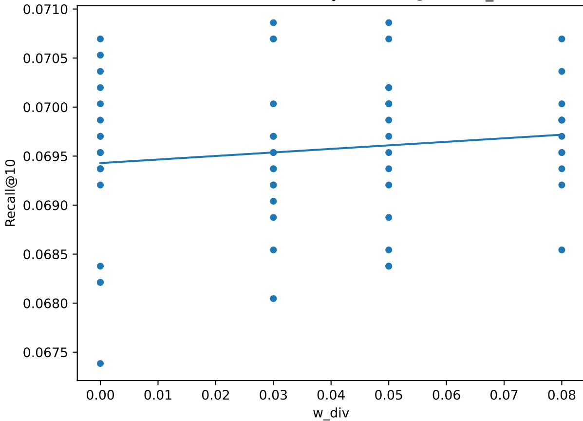
NGCF-Rerank: Sensitivity of Recall@10 to w_div
