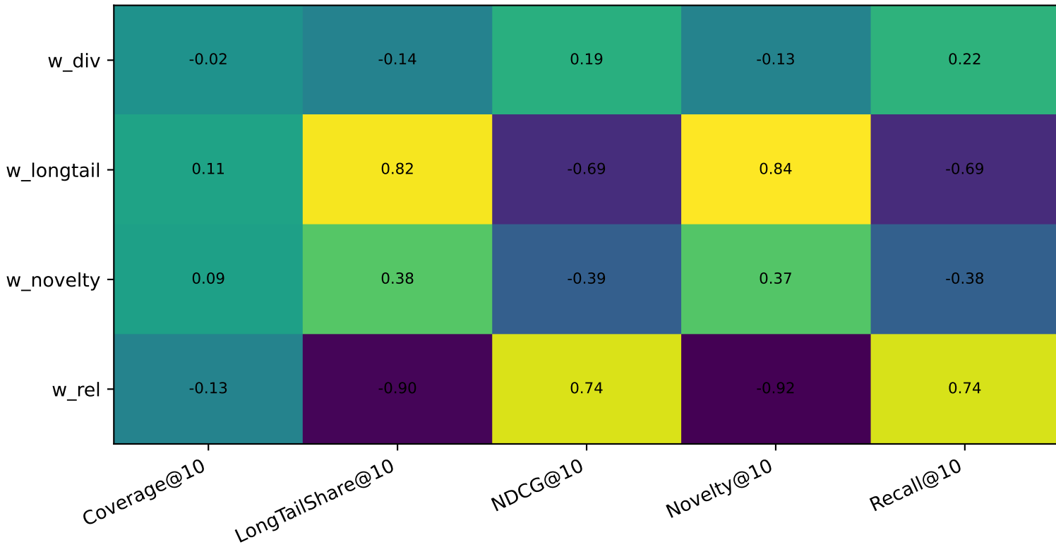
Mean Pearson Correlation: Weight vs Metric (across models)
