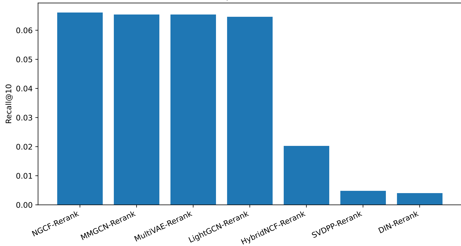
Model Comparison on Recall@10
