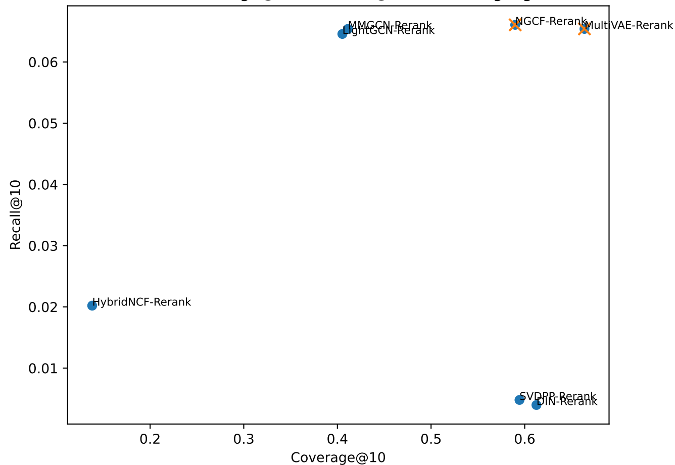
Trade-off: Coverage@10 vs Recall@10 (Pareto highlighted)
