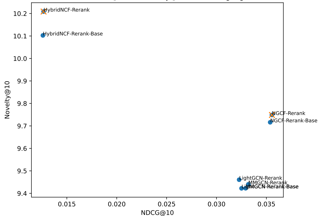
Trade-off: NDCG@10 vs Novelty@10 (Pareto highlighted)
