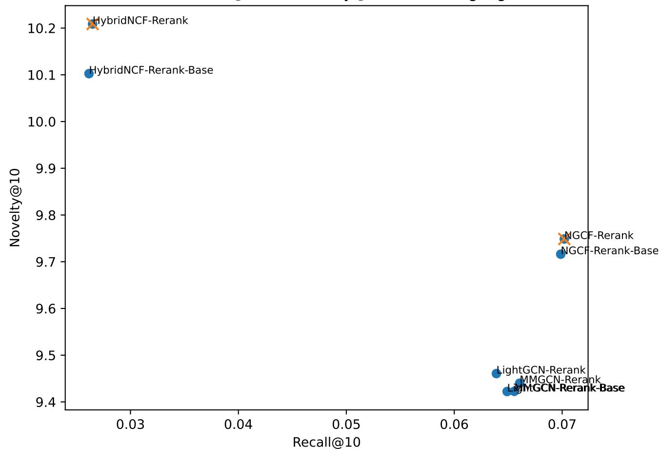
Trade-off: Recall@10 vs Novelty@10 (Pareto highlighted)
