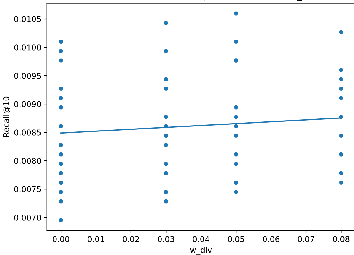
SVDPP-Rerank: Sensitivity of Recall@10 to w_div
