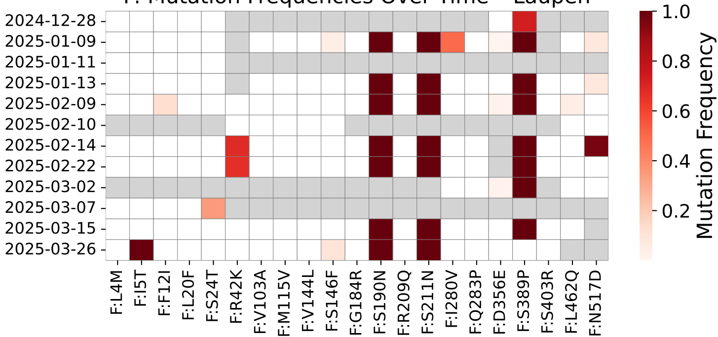
F: Mutation Frequencies Over Time – Laupen
