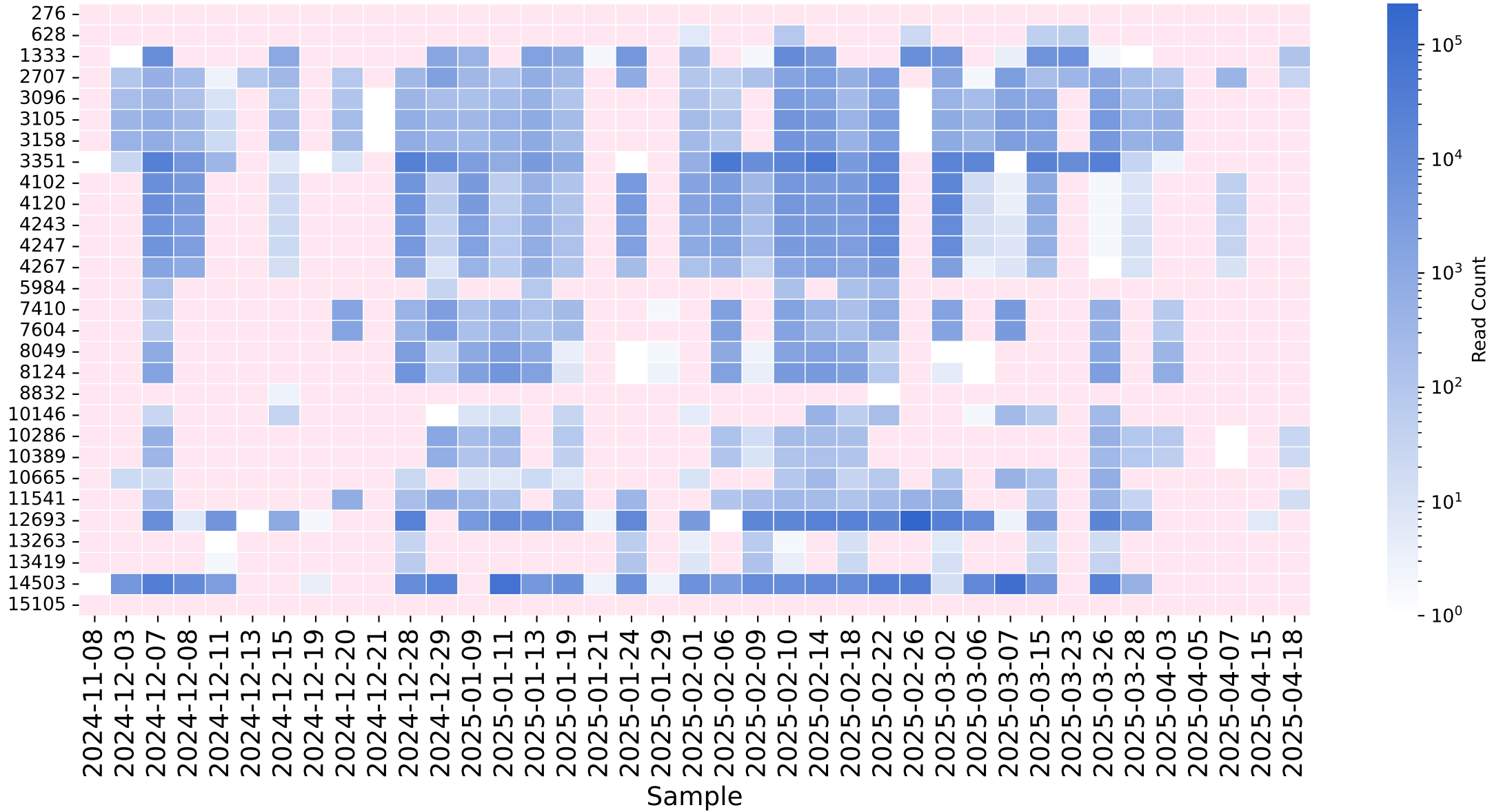
Coverage at unique B.D.E.1.1 mutations - Lugano
