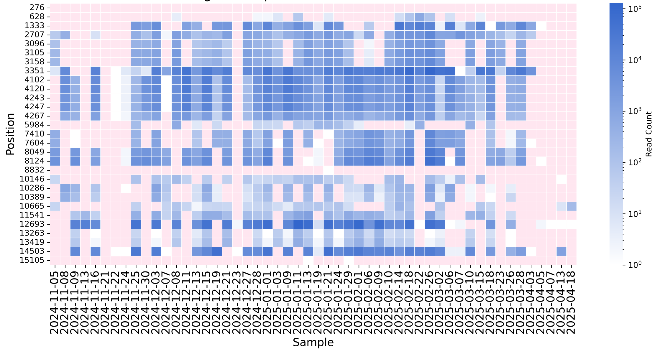
Coverage at unique B.D.E.1.1 mutations - Zurich
