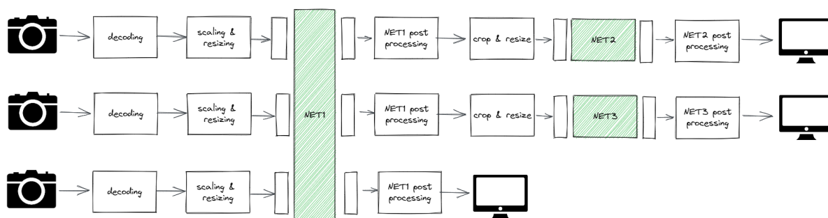
Figure 15. Stream Multiplexer
