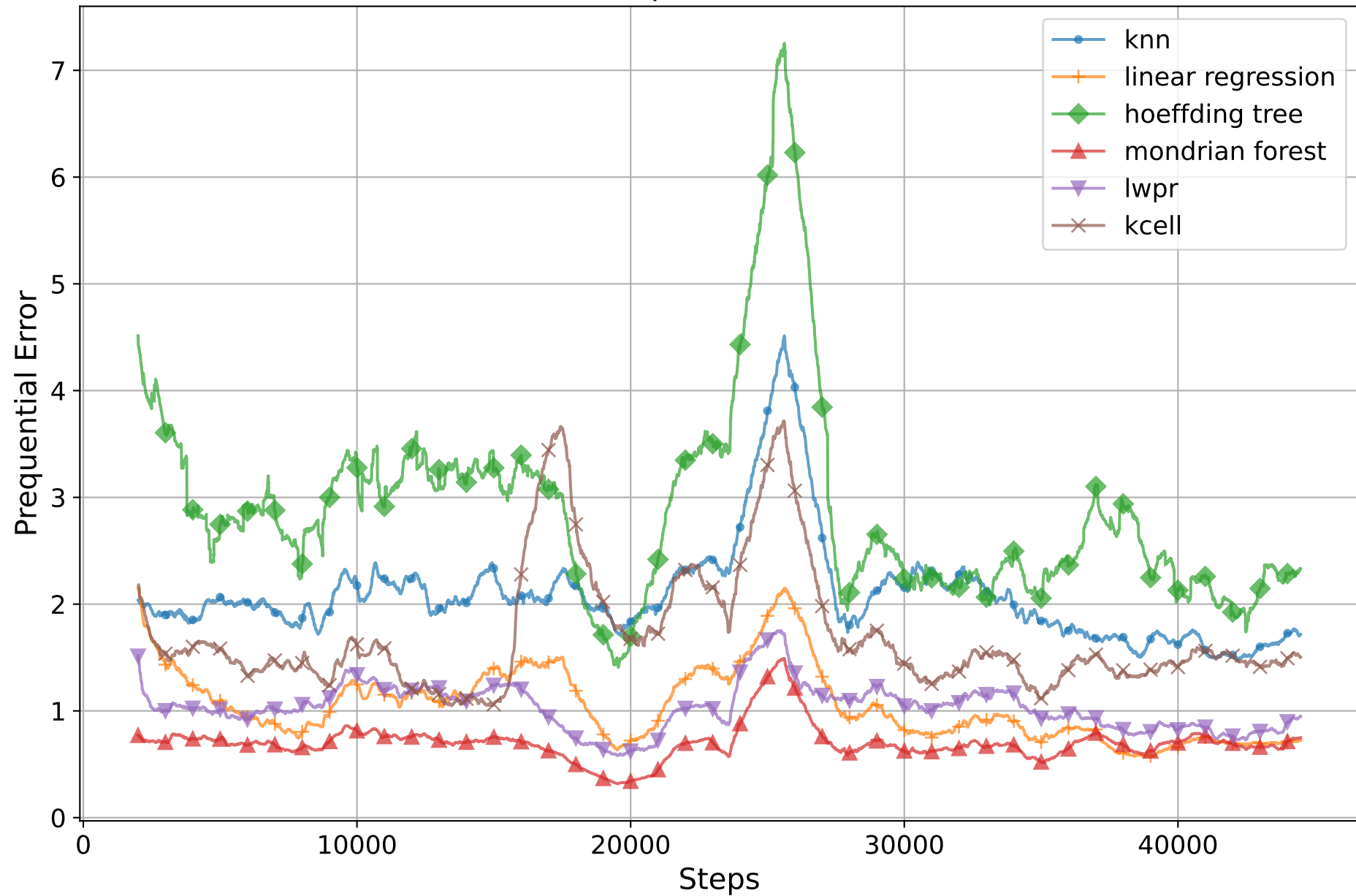
Smoothed Prequential Error (w=2000)
