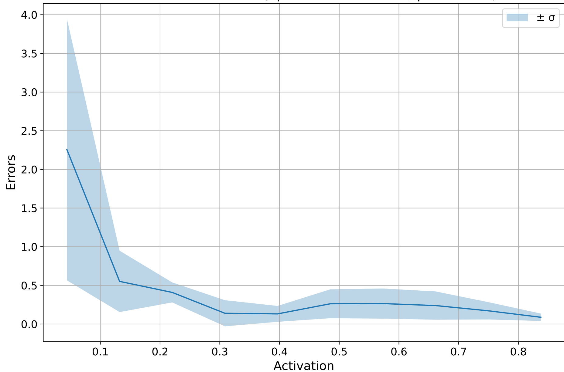
Test Error vs Activation (Spearman corr=-0.68, p=0.0e+00)
