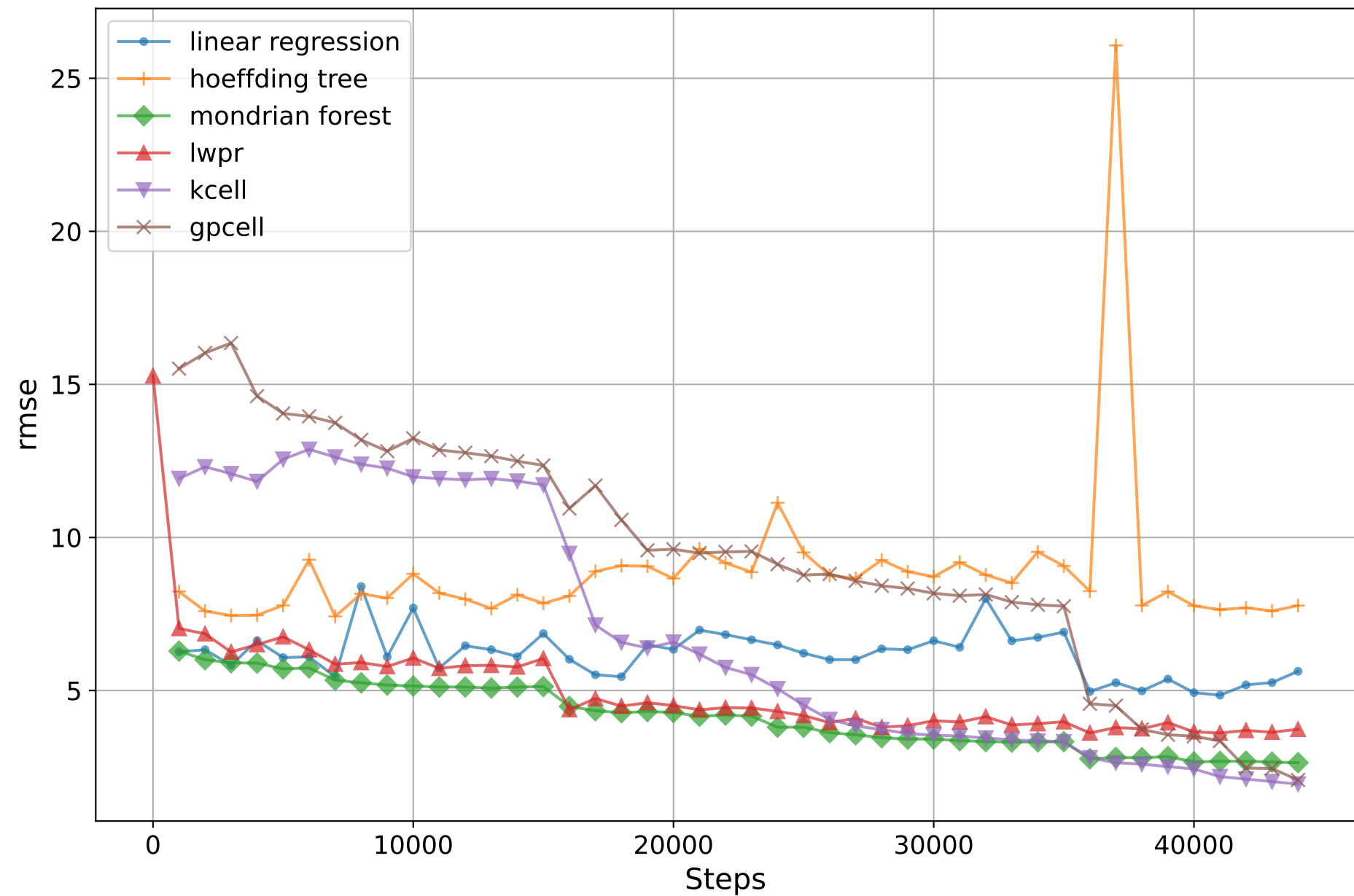
RMSE on Test Set
