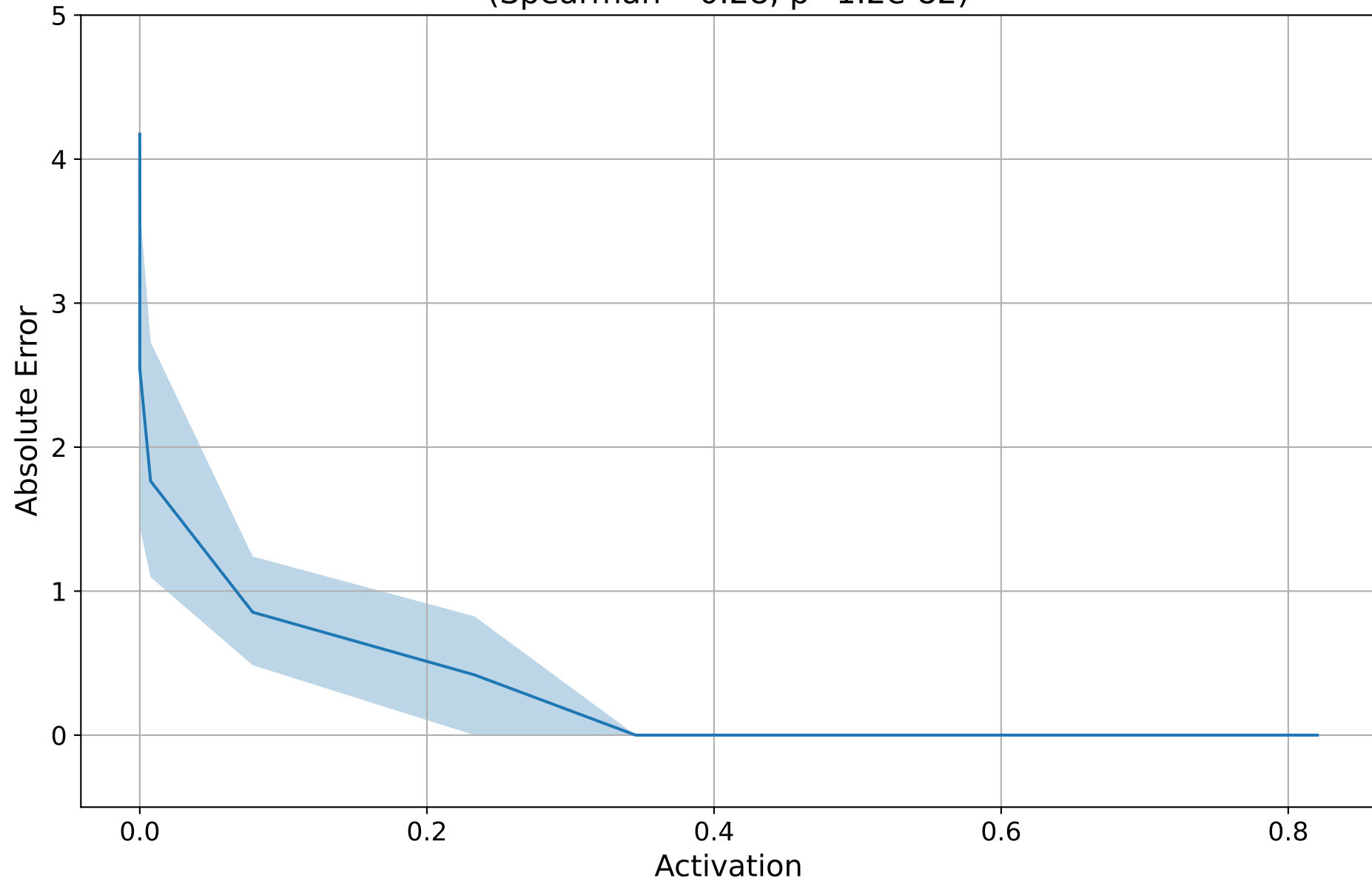
Prediction Error vs. Activation Value of Closest Agent (Spearman=-0.28, p=1.2e-82 )
