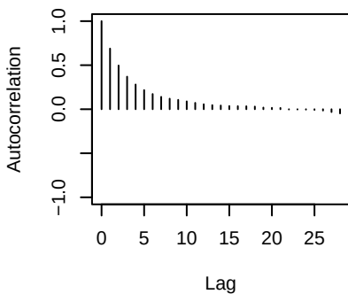
lambda[4]
