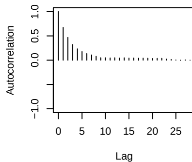
lambda[3]
