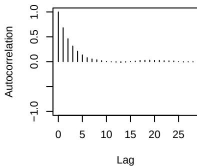
lambda[2]
