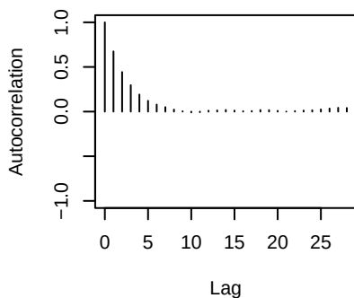
lambda[8]
