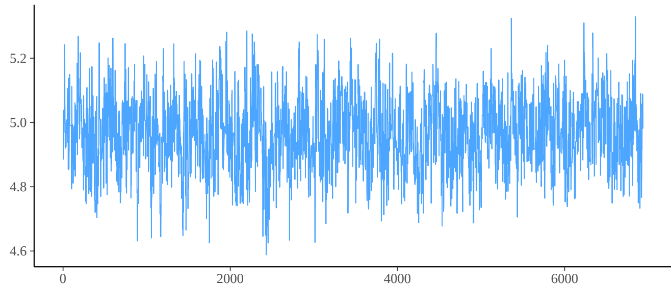
lambda[2]
