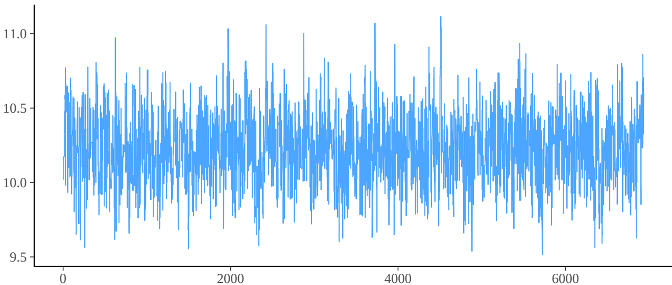
lambda[1]
