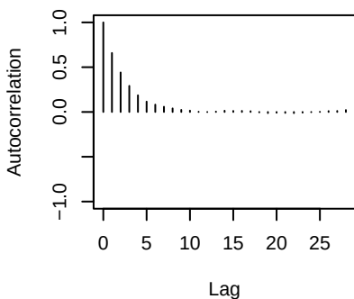
lambda[7]
