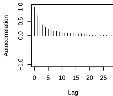
lambda[6]
