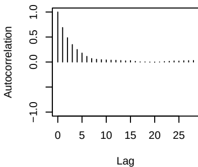
lambda[1]
