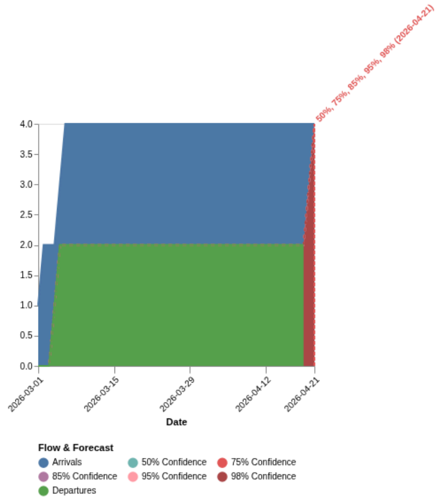
Forecasted Cumulative Flow Diagram
