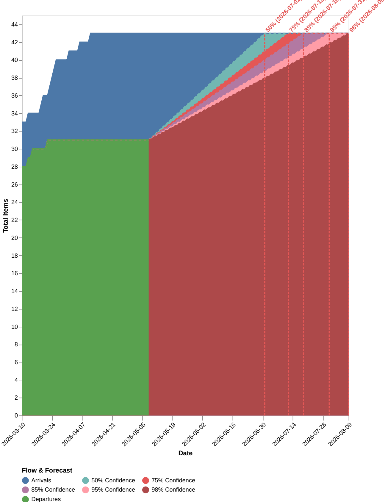
Forecasted Cumulative Flow Diagram
