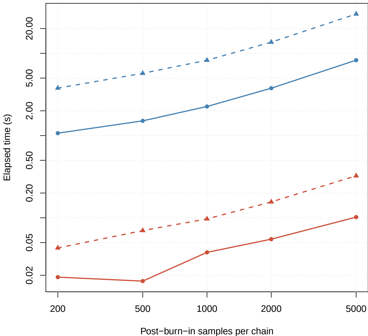
MCMC sample size vs fitting time
