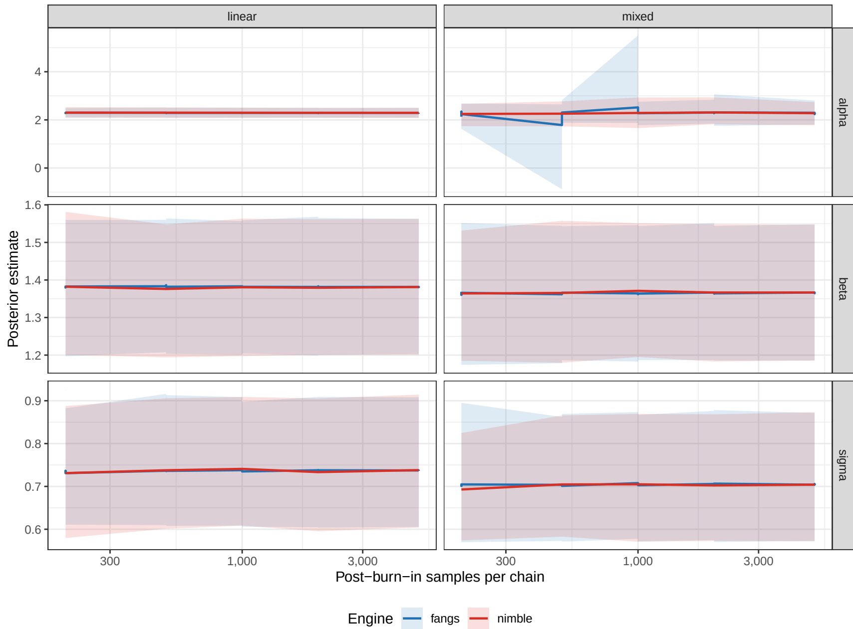
Posterior means & 95% CIs vs MCMC sample size
