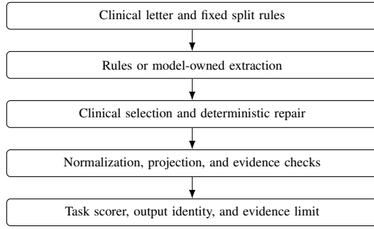
Fig. 1. Processing steps and their owners. Ownership remains explicit when a step is implemented by an LLM.
