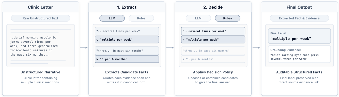
Fig. 2: A clinic letter passes through two stages (extract, then decide) to produce a structured label with grounding evidence. Either stage can be performed by an LLM or by rules; the highlighted choices show the Hybrid configuration.
