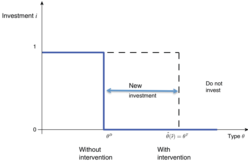
FIGURE 2. EQUILIBRIUM INVESTMENT
