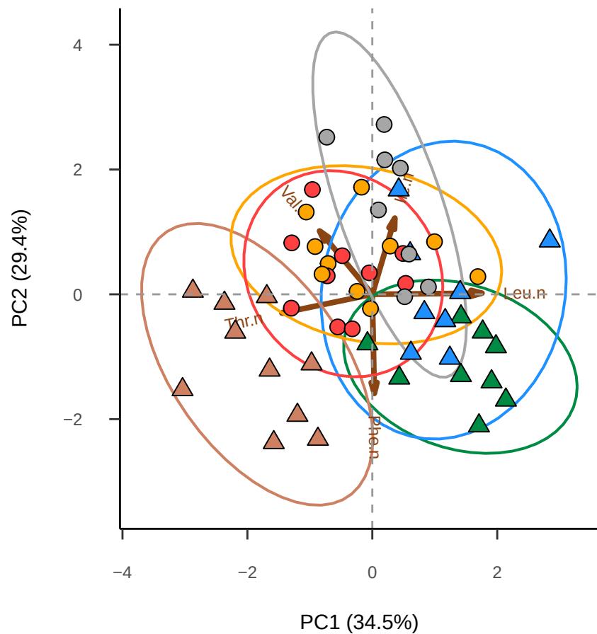
A ESS-normalized
