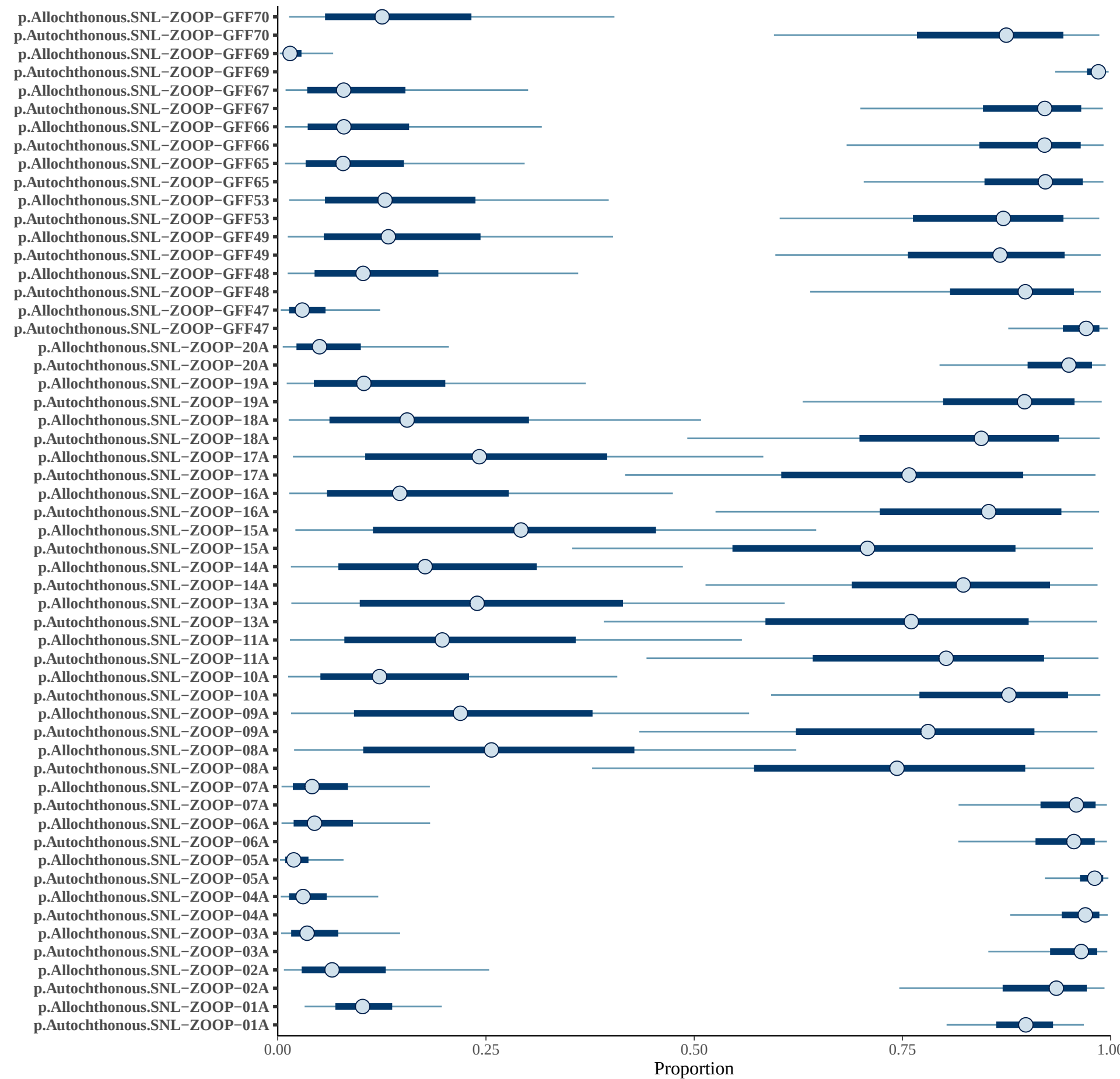
Proportions by SampleID
