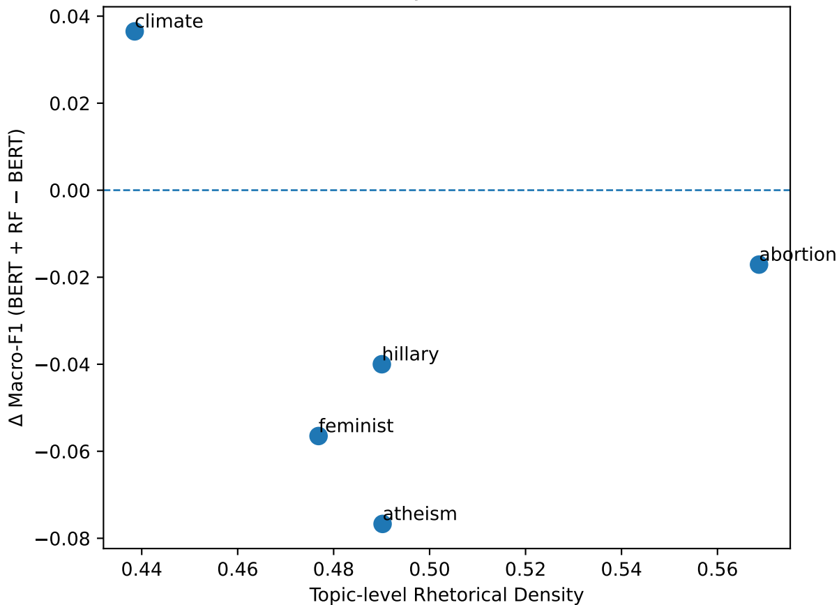
Rhetorical Density vs. Performance Gain
