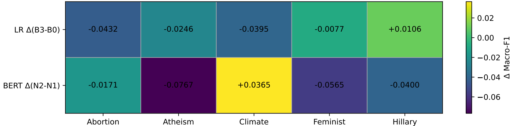
Topic \times \Delta Macro-F1 (Rhetorical Features vs Text-only)
