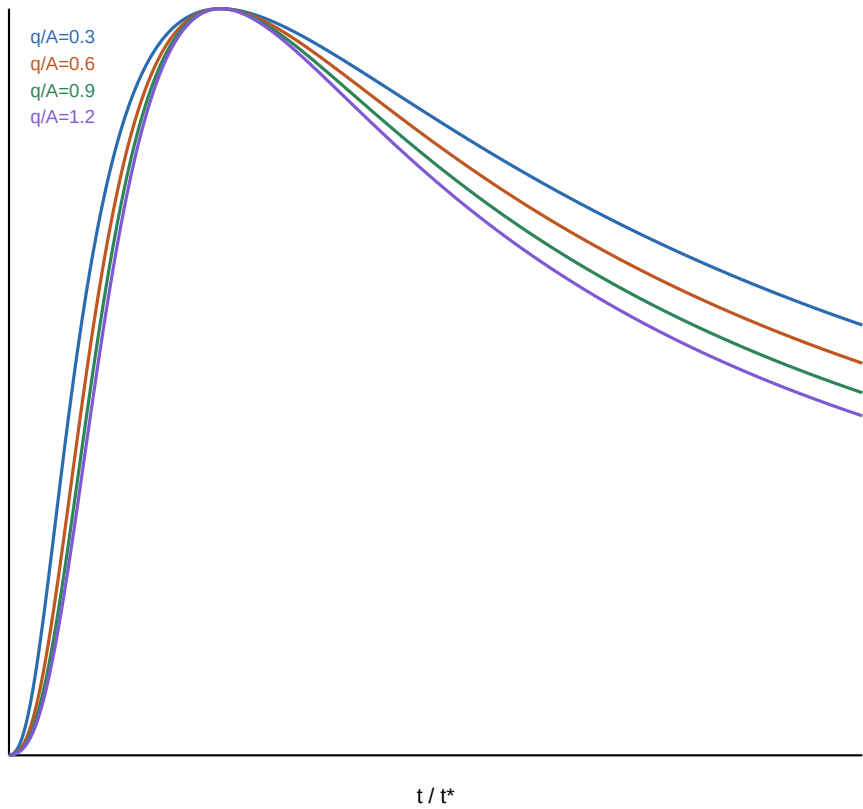
E. Peak collapse
