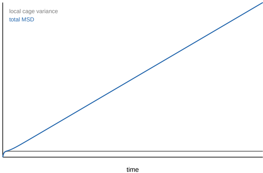
A. MSD: cage plateau followed by renewal diffusion
