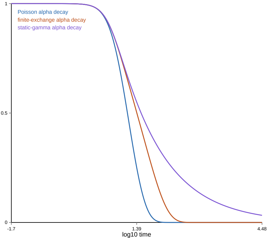
S. Static disorder broadens alpha decay
