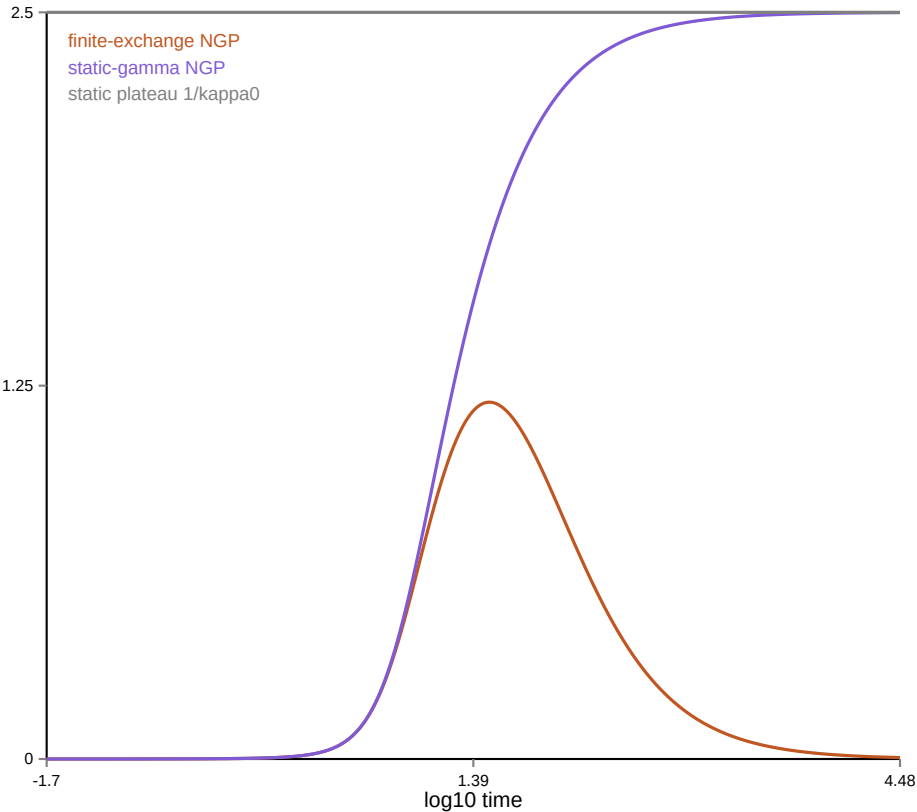
T. Static disorder lacks Gaussian recovery
