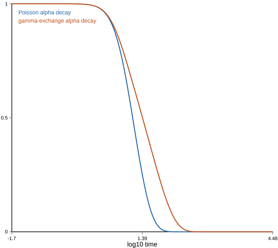
O. Alpha relaxation from renewal heterogeneity
