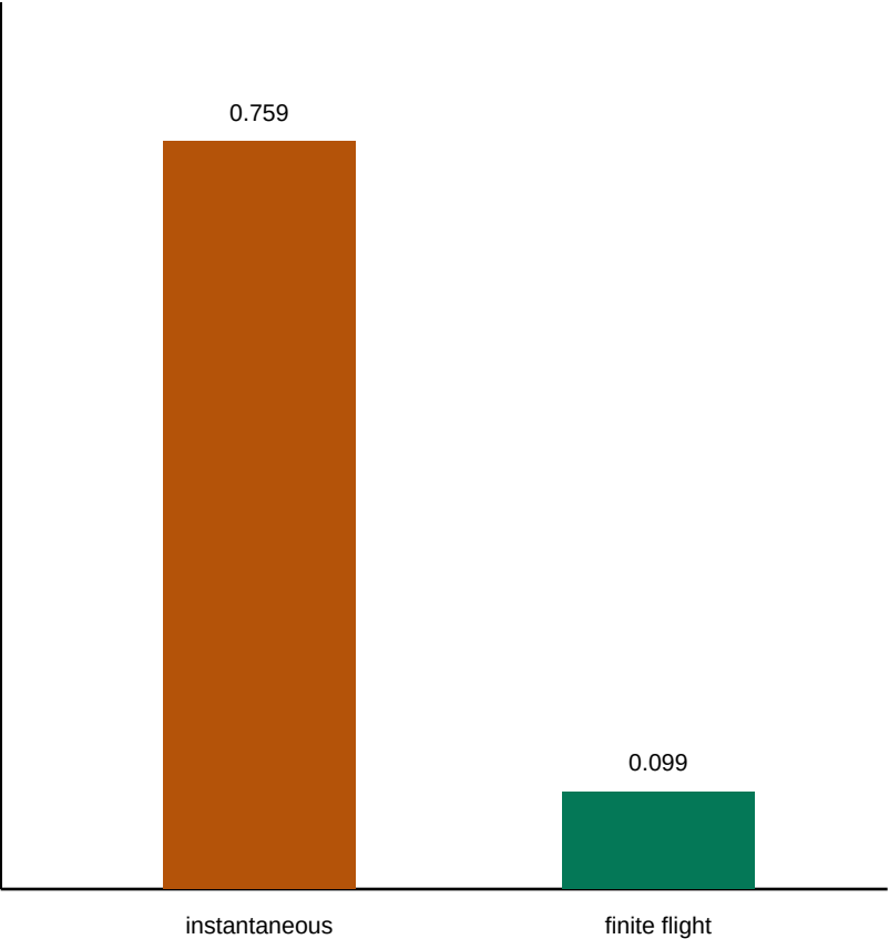
B. T=0.58 transient NGP absolute error
