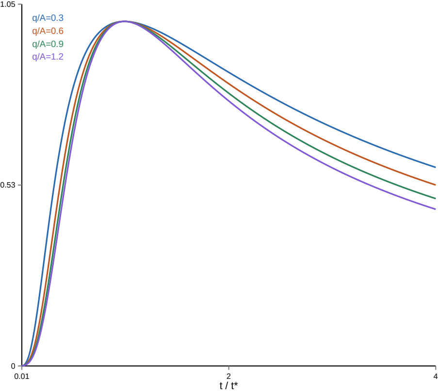
E. Peak collapse
