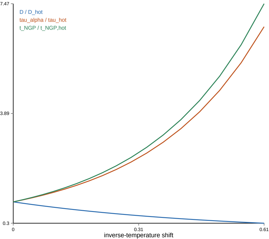
I. Transport and relaxation decouple on cooling
