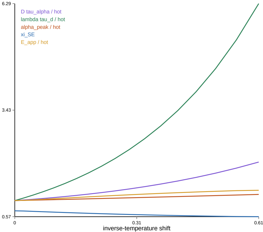
J. Stokes-Einstein product and delayed-renewal control
