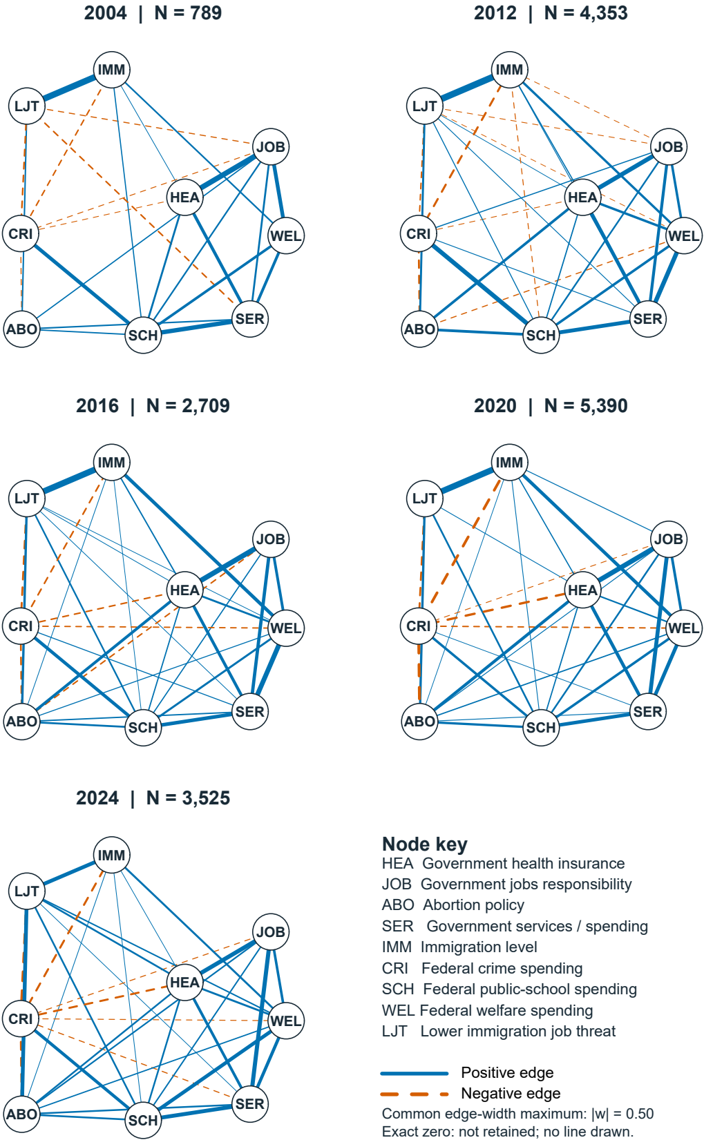
Figure 4.1 Policy-attitude networks across five election years
