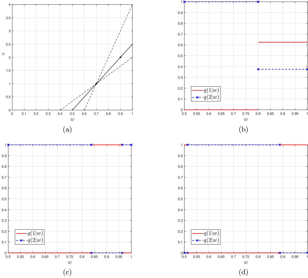
Figure 3: (a) Illustration of the two receivers' lines, \ell_1(w; \mu_1^*) and \ell_2(w; \mu_2^*) (solid), which completely overlap and pass through points (0.7, 1) and (0.9, 2) , along with lines \eta_1 and \eta_2 from Theorem C.2 (dashed). (b) A randomized optimal persuasion mechanism, where q(1|w) = 5/8 for w \in [0.8, 1] , q(2|w) = 3/8 for w \in [0.8, 1] , and q(2|w) = 1 for w \in [0.5, 0.8] . (c) A deterministic optimal persuasion mechanism, where q(1|w) = 1 for w \in [0.8375, 0.9625] (centered around 0.9 and with length 1/8 ) and q(2|w) = 1 for w \in [0.5, 0.8375] \cup [0.9625, 1] . (d) A deterministic optimal persuasion mechanism, where q(2|w) = 1 for w \in [0.5125, 0.8875] (centered around 0.7 and with length 3/8 ) and q(1|w) = 1 for w \in [0.5, 0.5125] \cup [0.8875, 1] .
