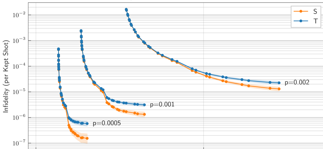
End-to-End Magic State Cultivation: d=3 b=Y , c=\text{end2end-inplace-distillation} , d_2=15 , \text{noise}=\text{uniform} , r_2=5
