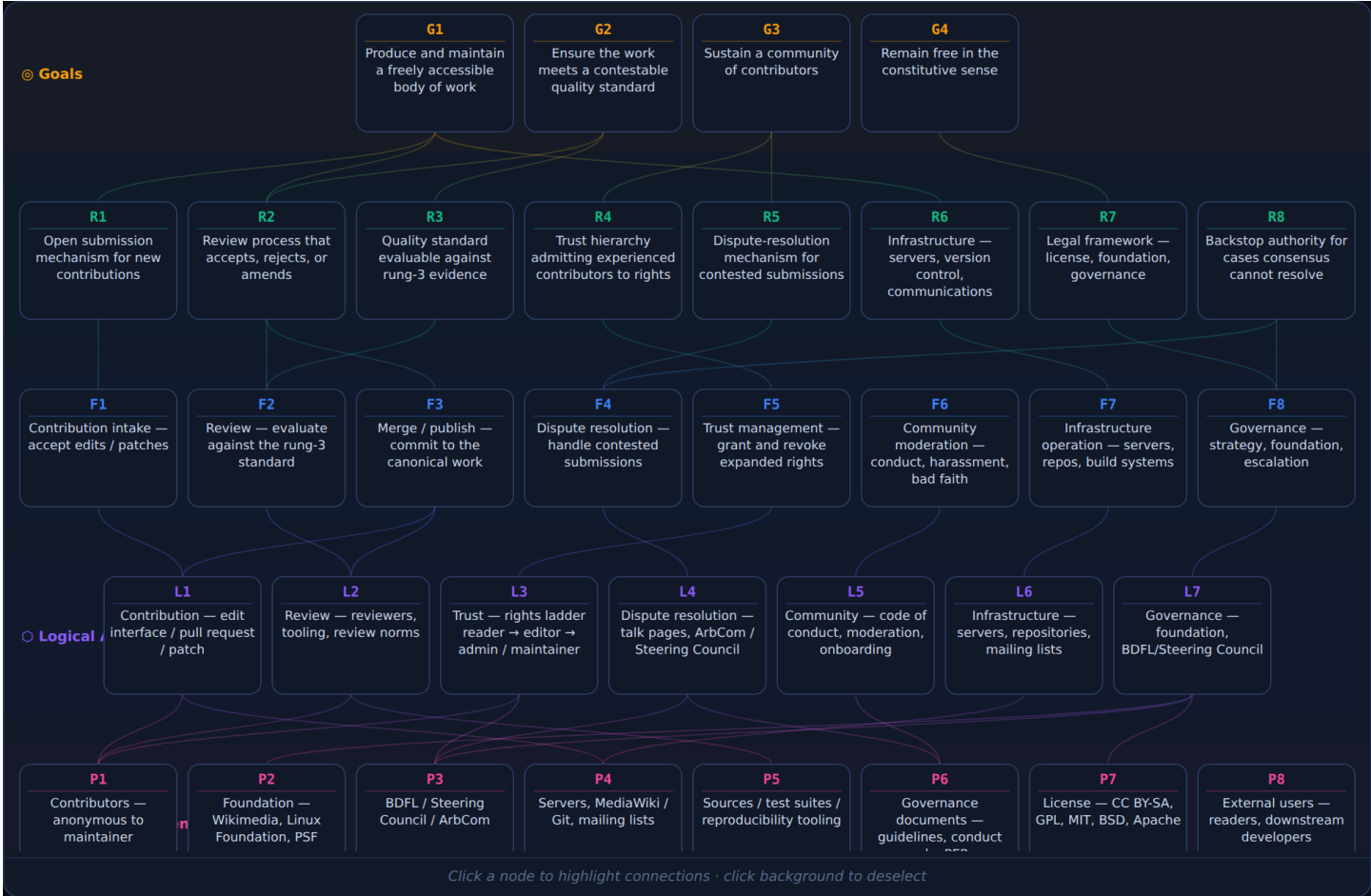
wikipedia — Graph
