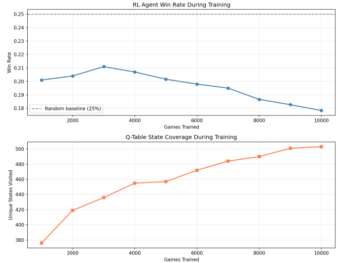
Fig. 3. RL Agent win rate and Q-table state coverage during training.
