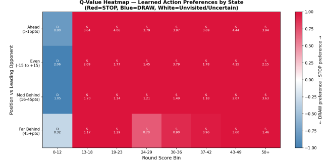
Fig. 5. Q-value heatmap showing learned action preferences by score bin and competitive position.
