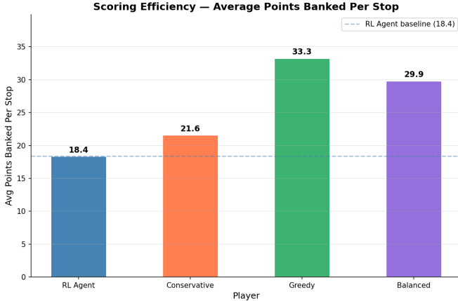
Fig. 4. Average points banked per stop across all agents.
