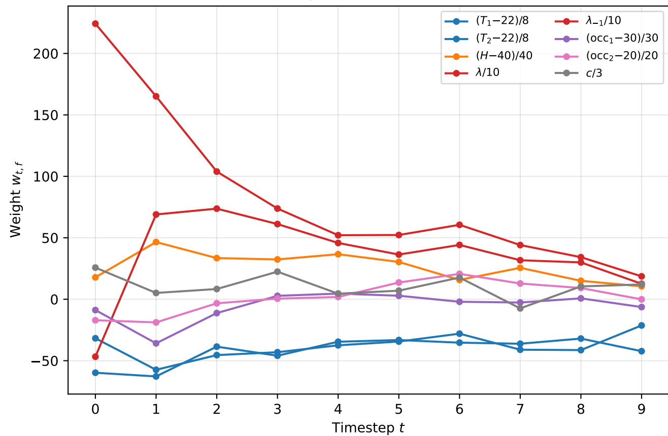
VFA weights \mathbf{w}_t — features 0-7
