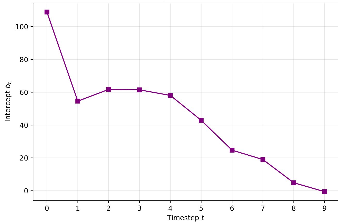
Ridge intercept b_t
