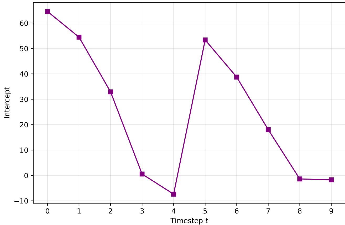
Intercept \eta_{t,6}
