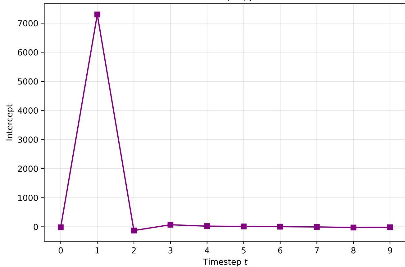
Intercept \eta_{t,6}
