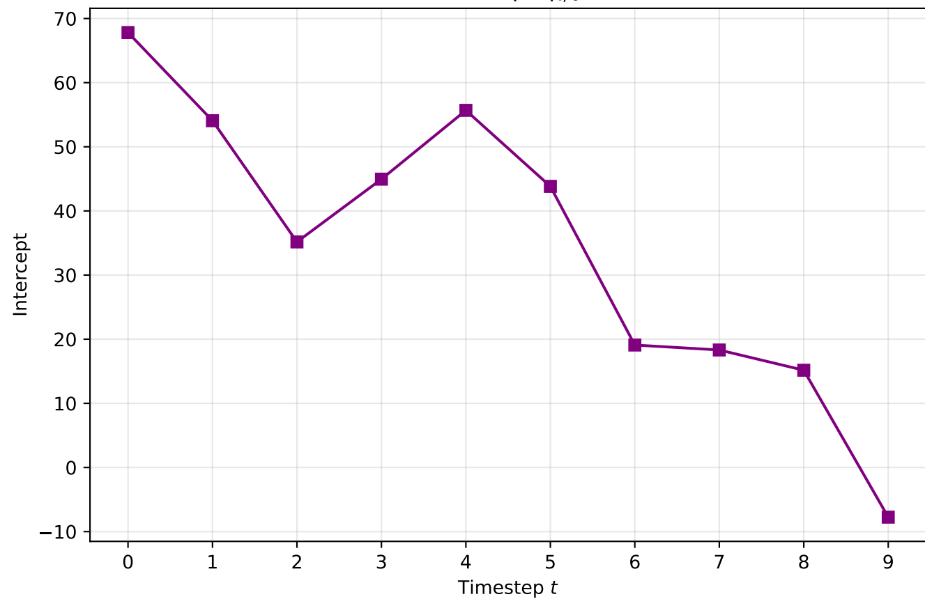
Intercept \eta_{t,6}
