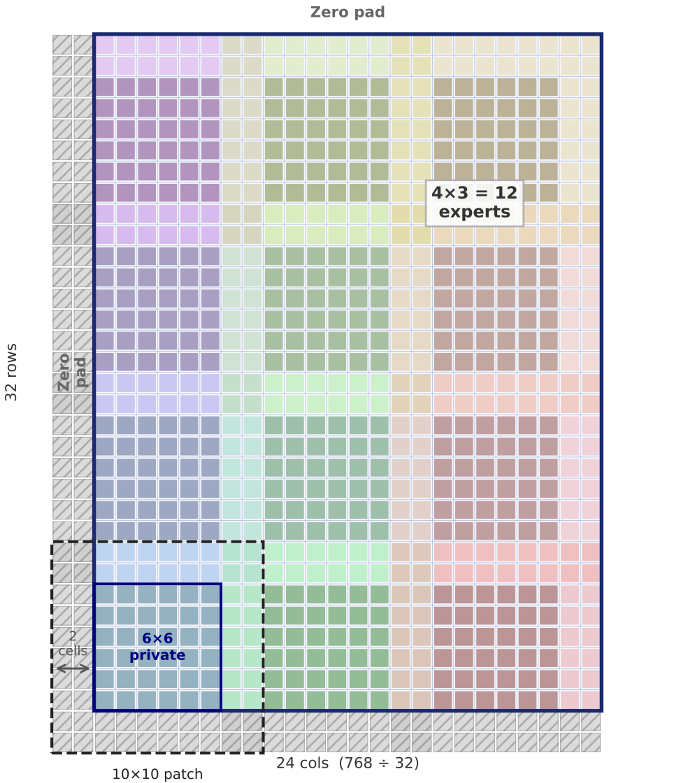
Architecture 04 — Flat Grid Overlap Zero-padding at boundaries
