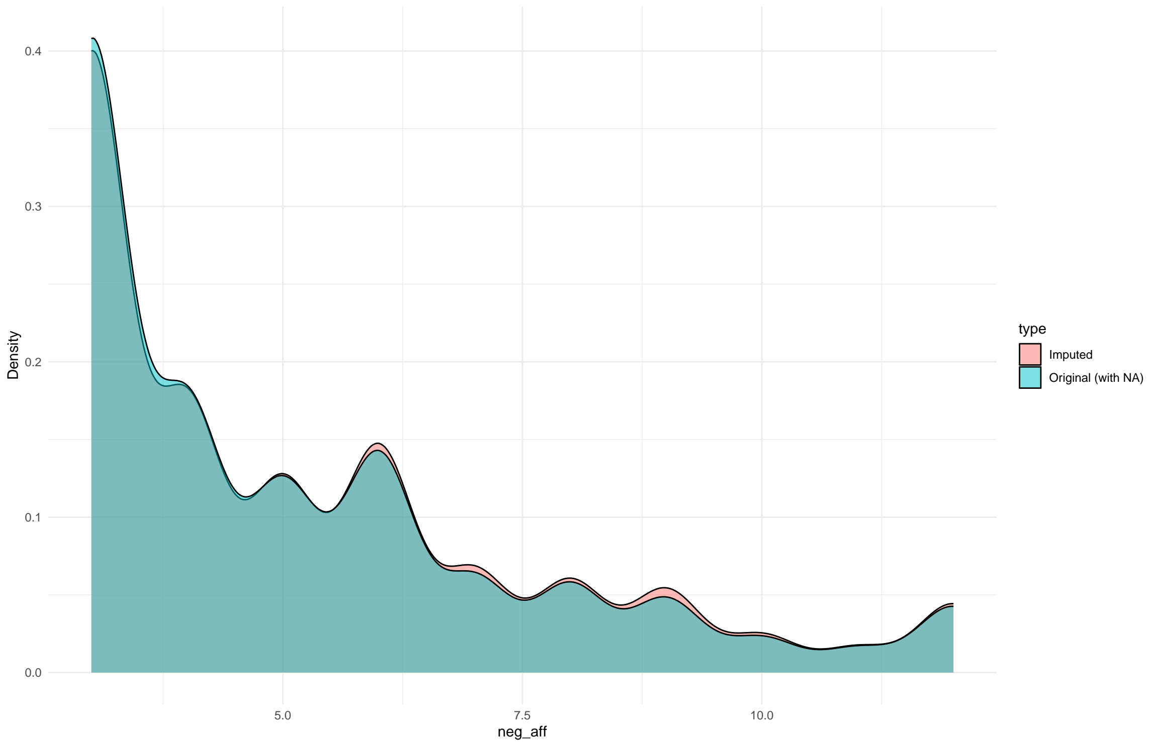
Distribution comparison: neg_aff
