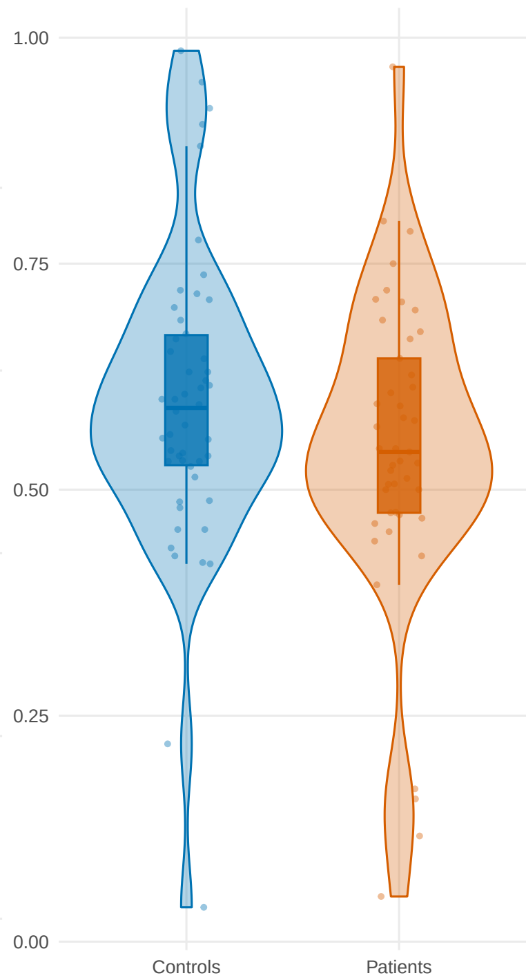
lose_shift
