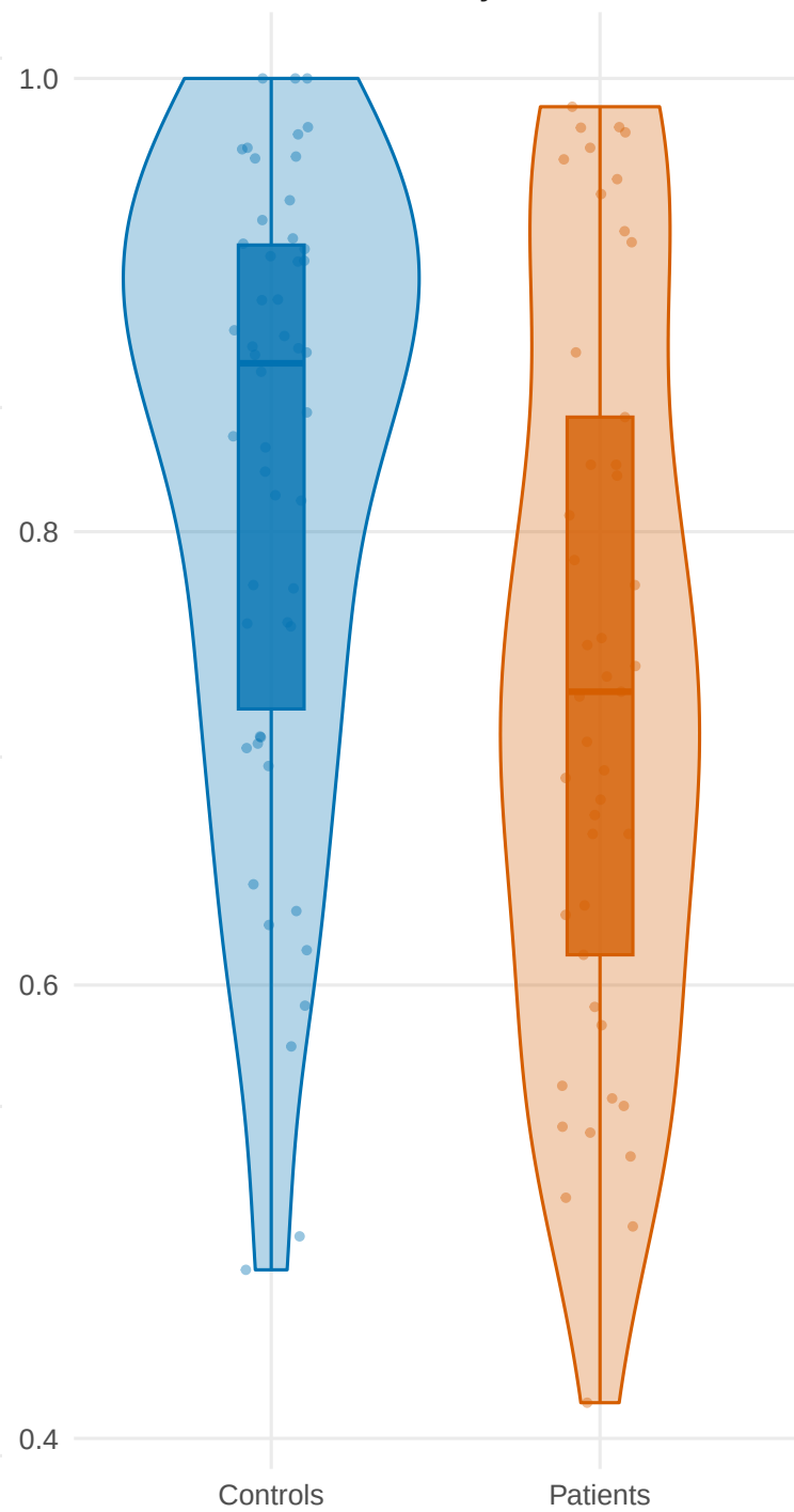
win_stay
