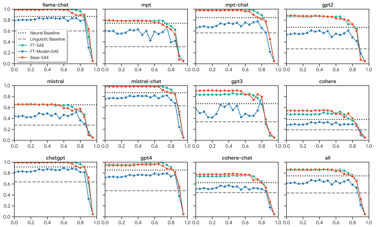
Figure 20: Recall at FPR=5% (y-axis) vs. Interpretability Threshold (x-axis) for L_1 -regularized logistic regression classifiers trained on the COLING dataset evaluated on various splits of the RAID dataset (Dugan et al., 2024).
