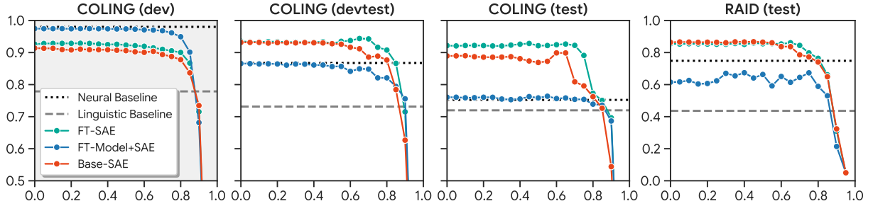
Figure 4: F1 Score (COLING) and TPR@FPR=5% (RAID) (y-axis) vs. Interpretability Threshold (x-axis) for classifiers trained on the COLING Shared Task 1 dataset evaluated on ID (grey) and OOD (white) data. We see that FT-MODEL+SAE matches the performance of the underlying neural detector even at high interpretability thresholds (0.7+) and that BASE-SAE and FT-SAE models exceed the detector’s performance on OOD data.
