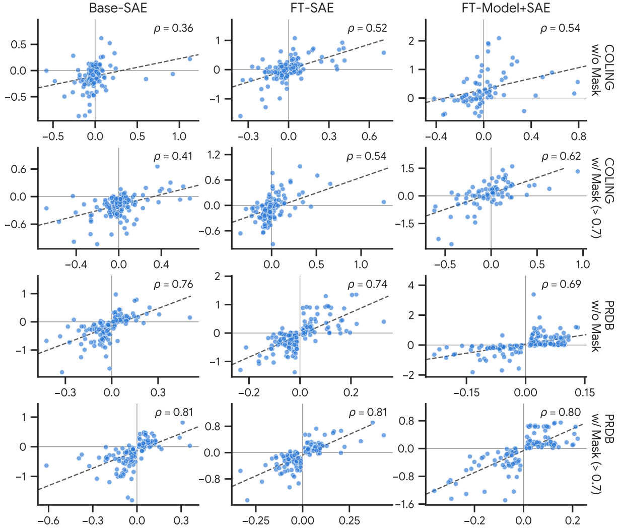
Figure 9: Per-feature agreement between the two interventions (§7), for the logistic-regression heads. Each point is one SAE feature. The x -axis is the feature’s mean change in the detector’s AI logit when the feature is zero-ablated, and the y -axis is the mean change when the text is instead paraphrased to remove the feature, both averaged over the documents in which the feature was sampled. Positive values on both axes mean the feature pushed the prediction toward AI and removing it from the text lowered the AI logit. Columns are the feature settings; the top two rows are COLING without and with the interpretability mask ( \tau > 0.7 ), the bottom two rows the same for PRDB (GPT-4o).
