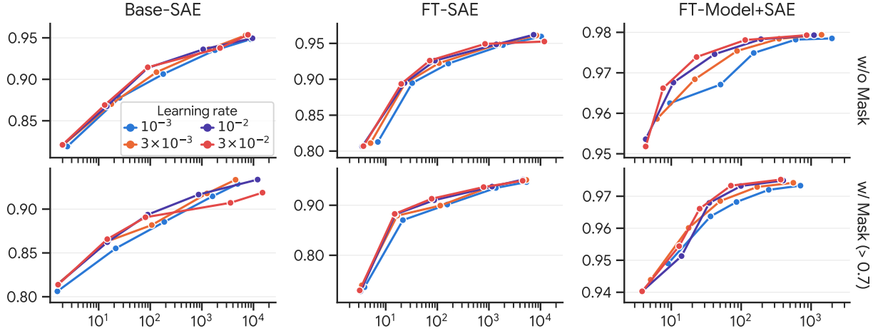
Figure 6: COLING-dev F1 against the mean number of active features per document (log scale) for the SGD + L_1 grid, three epochs. Columns are the feature settings, rows the mask thresholds; each line follows one learning rate through the five \lambda values (leftmost point \lambda = 1 , rightmost \lambda = 10^{-2} ).
