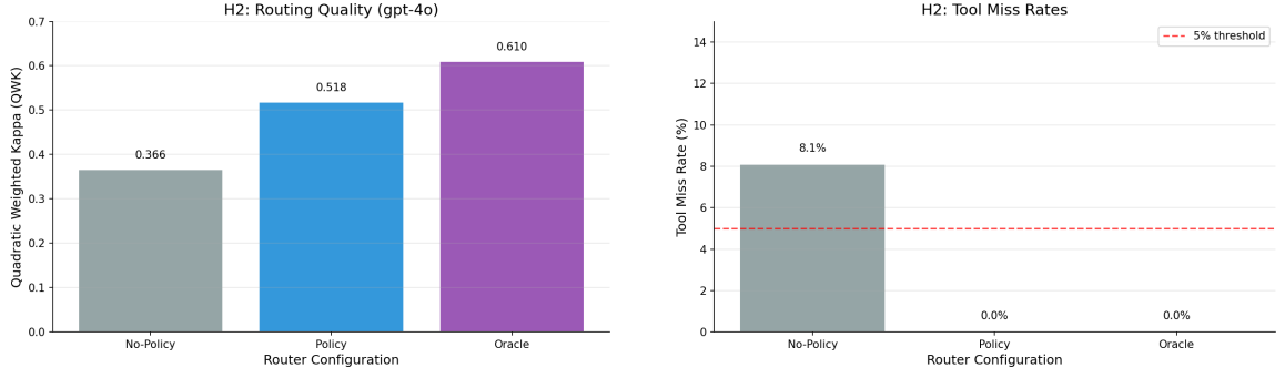
(a) QWK for gpt-4o under three routing configurations: no-policy, LAMINA Policy router, and oracle router.
