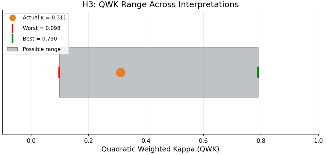
Figure 3.4: Range of possible QWK on vague claims for best vs. worst numeric remappings of ambiguous quantifiers.
