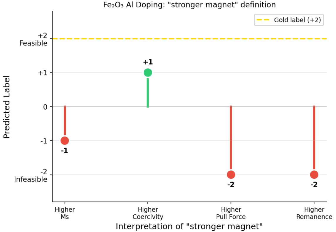
Figure 3.8: Ambiguity-induced flips for the \text{Fe}_2\text{O}_3 Al-doping claim (“Someone made a stronger magnet by doping \alpha\text{-Fe}_2\text{O}_3 with Al”). Interpreting “stronger magnet” as higher M_s , higher coercivity, higher pull force, or higher remanence yields predicted labels of -1 , +1 , -2 , and -2 , respectively, for a gold label of +2 .
