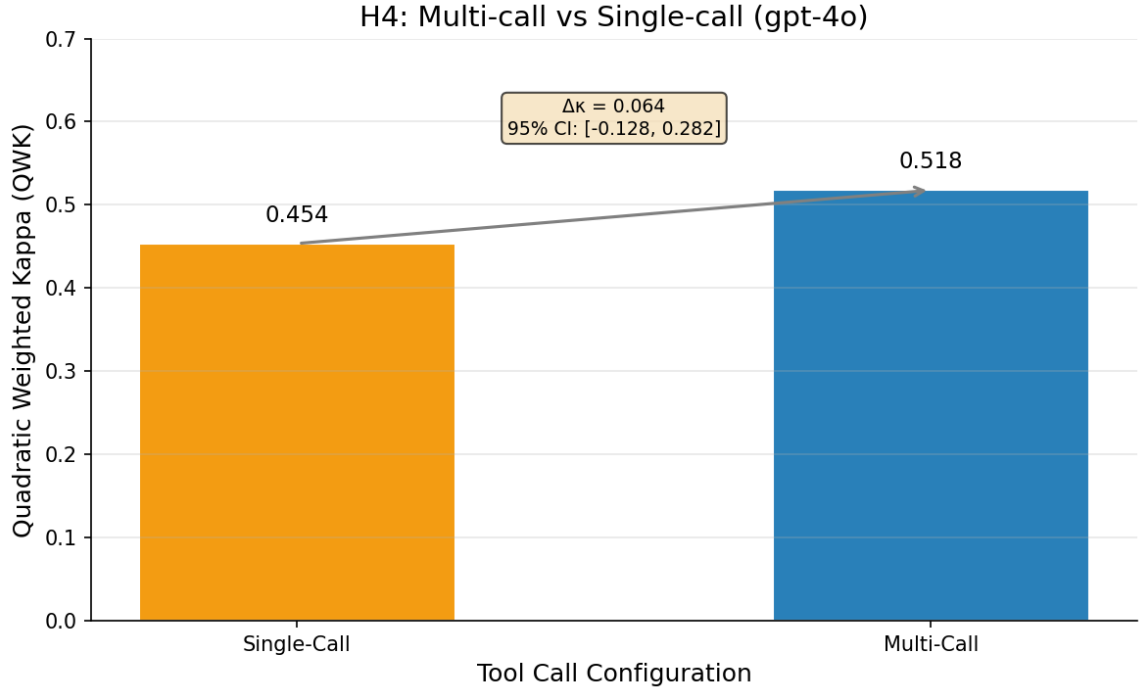
Figure 3.5: Agreement (QWK) for gpt-4o with tools under single-call vs. multi-call settings. Arrow annotation shows \Delta\kappa and its 95% confidence interval.
