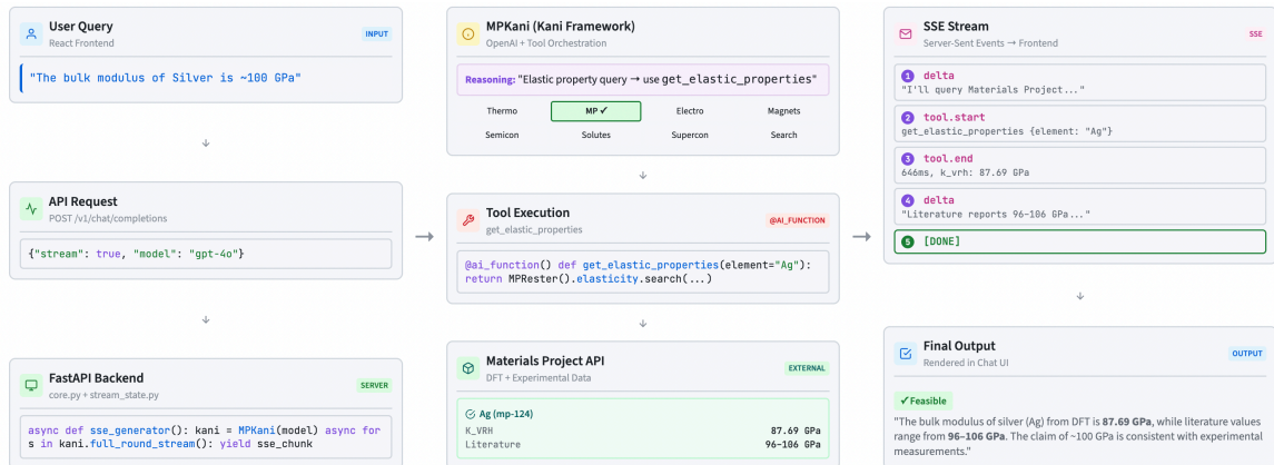
Figure 2.2: Backend architecture and tool orchestration. FastAPI hosts a Kani-based controller that selects tools, calls external services (CALPHAD, Materials Project, CHGNet, etc.), and emits SSE traces for each interaction.
