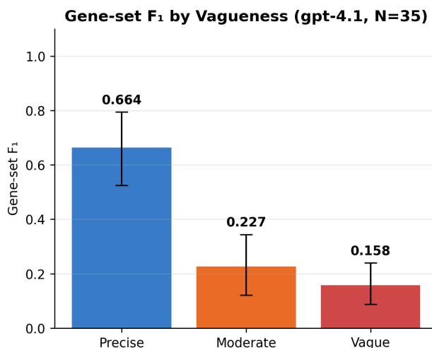
Figure 5.2: Gene-set F_1 by prompt vagueness (gpt-4.1, N = 35 ). Error bars show 95% bootstrap CIs. The precise–moderate gap is the dominant transition.
