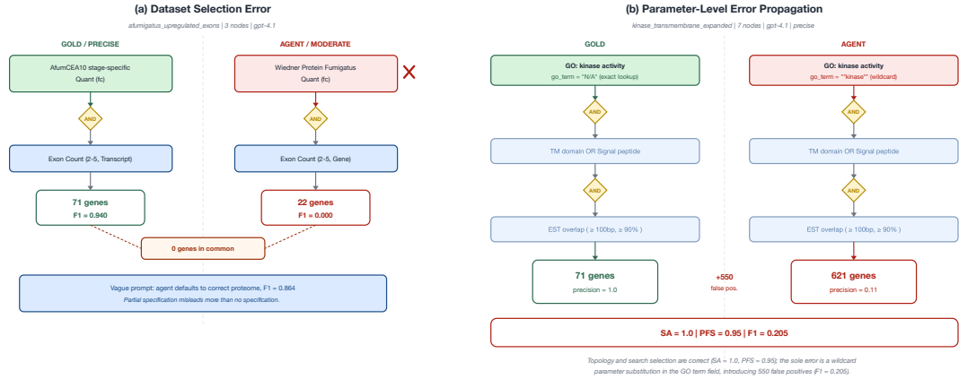
Figure 5.7: Two failure modes from real evaluation runs (gpt-4.1). (a) Dataset selection error: the moderate prompt causes the agent to select a different proteomics experiment (Wiedner vs. AfumCEA10) for a 3-node strategy, producing zero gene overlap despite correct tree structure. The vague prompt defaults to the correct dataset ( F_1 = 0.864 ). (b) Parameter-level error propagation: the agent builds the identical 7-node tree as the gold (SA = 1.0, PFS = 0.95), but a single wildcard substitution in the GO term field ("*kinase*" instead of "N/A") inflates the gene set from 71 to 621, producing 550 false positives ( F_1 = 0.205 ).
