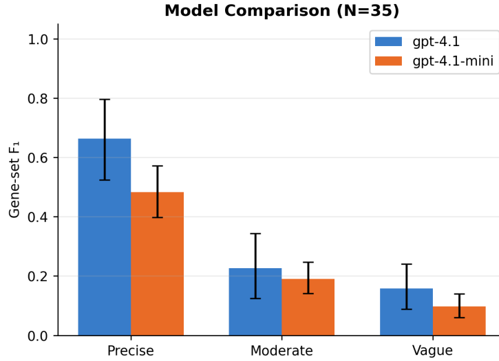
Figure 5.6: Gene-set F_1 for gpt-4.1 ( N = 35 ) vs. gpt-4.1-mini (mean of 3 replicates, N = 35 ) at each vagueness level. The vagueness gradient replicates on the smaller model, with the gap largest for precise prompts.
