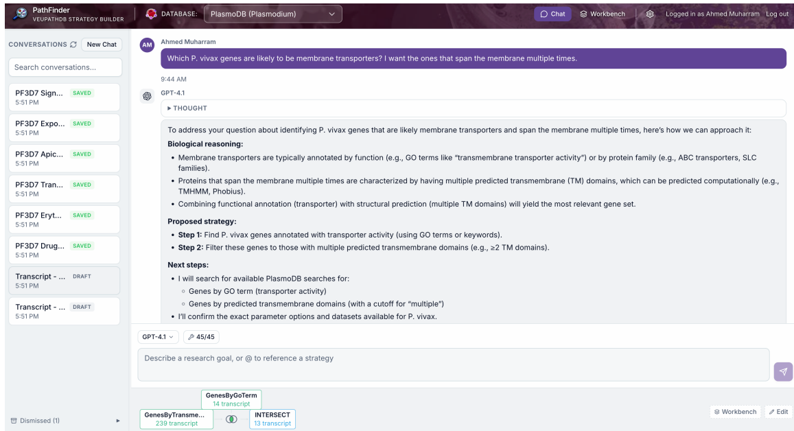
Figure 4.2: PathFinder’s interface during strategy construction for the pvivax_tm_transporter strategy. The conversation panel shows the agent’s reasoning and proposed strategy, while the bottom bar displays the minimized strategy graph: a GenesByGoTerm leaf node and a GenesByTransmembraneDomains leaf node joined by an intersection operator.
