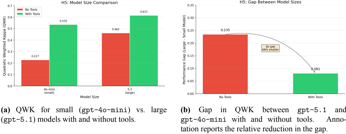
Figure 3.6: H5: Model size and diminishing returns with tools on Drop-4.
