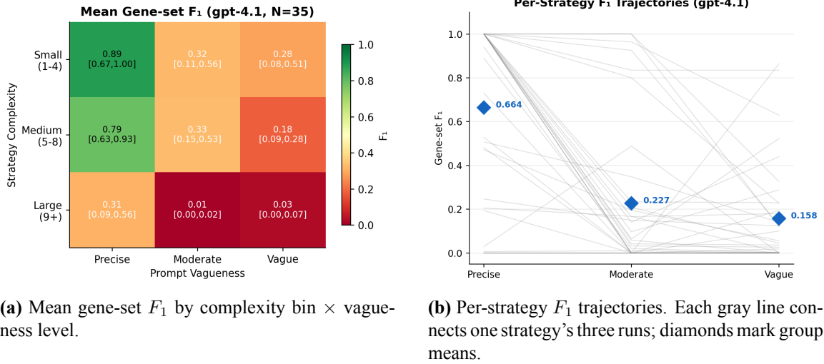
Figure 5.5: H2: Complexity and vagueness compound (gpt-4.1, N = 35 ). (a) Both factors independently degrade performance; their combination produces near-total failure. (b) Most strategies drop steeply from precise to moderate, with several large strategies near zero across all conditions.
