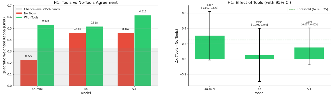
(a) QWK for each model with and without tools on Drop-4. The shaded band indicates the 95% chance-level region.
