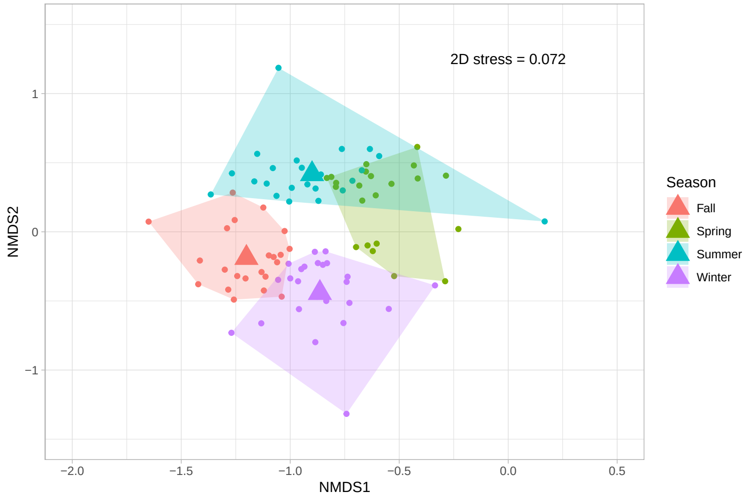
NMDS of Species by Season
