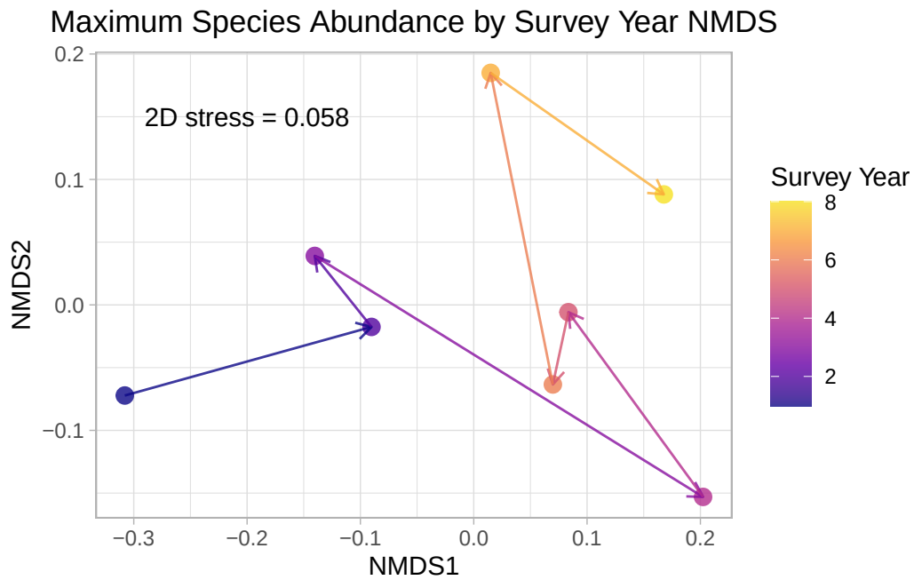
Figure 2: Replication of the ‘Maximum Species Abundance’ NMDS. I reproduced it thinking that with cleaner data it might appear differently, giving insight into species identity similarities or differences, following the bar chart of species richness. The usage of setdiff() may be more desirable in this situation. I became unsure of the application of setdiff() you (Francis) wrote on the sticky note and would love to revisit it.
