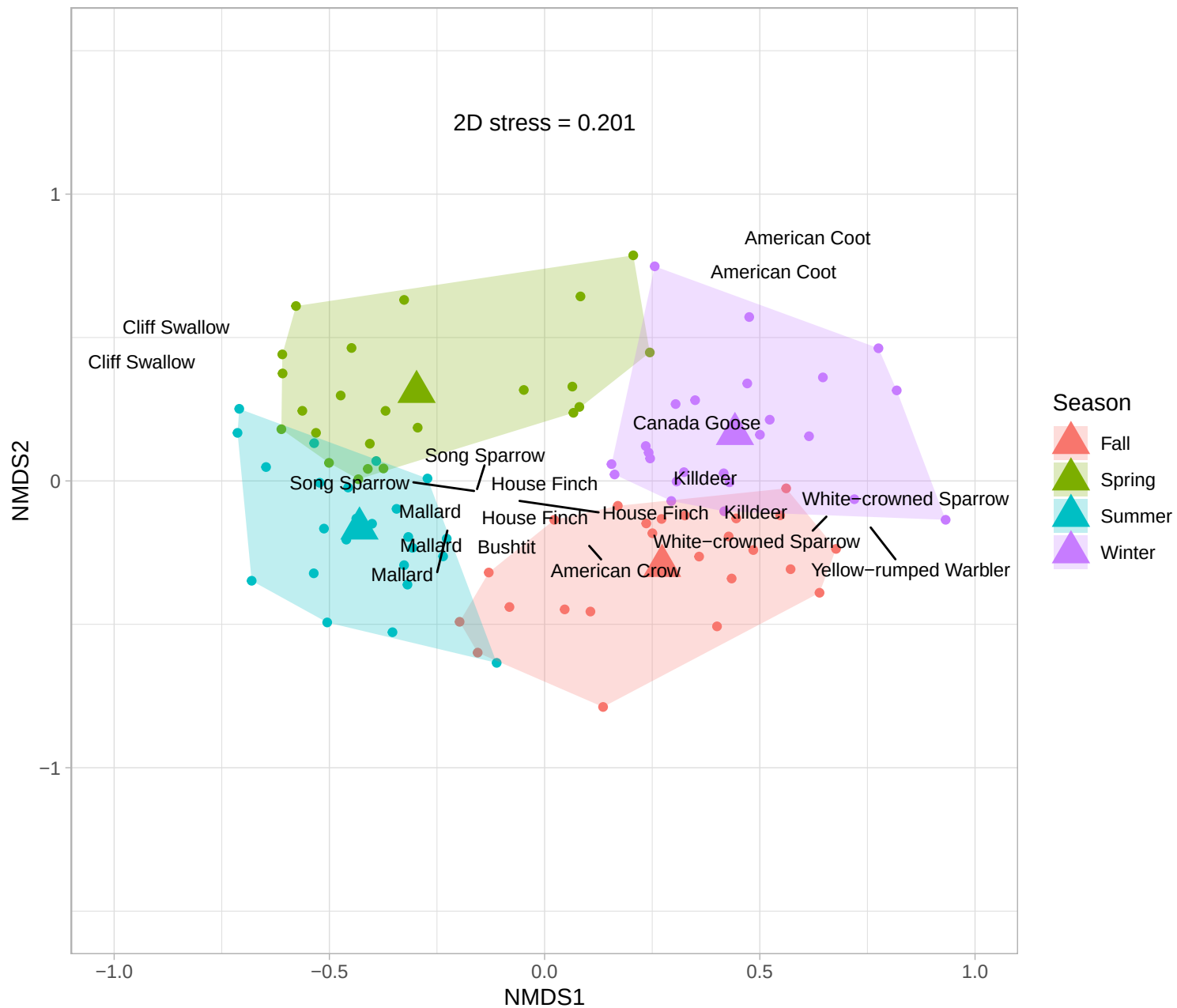
NMDS of Species by Season
