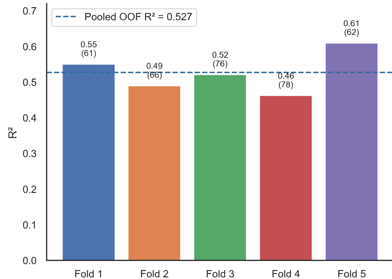
Performance remains positive in every source fold
