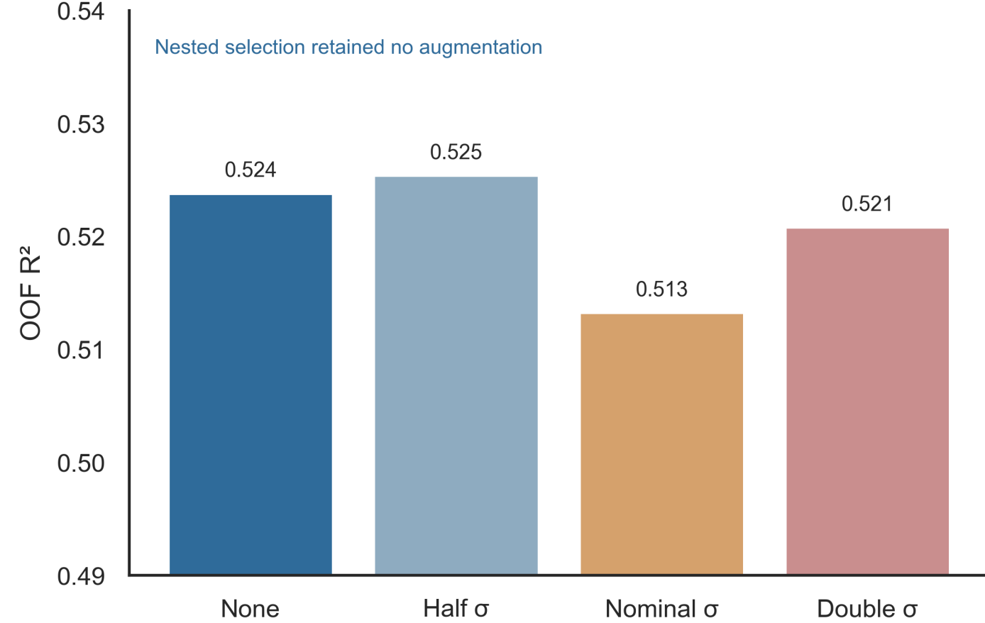
Augmentation decision
