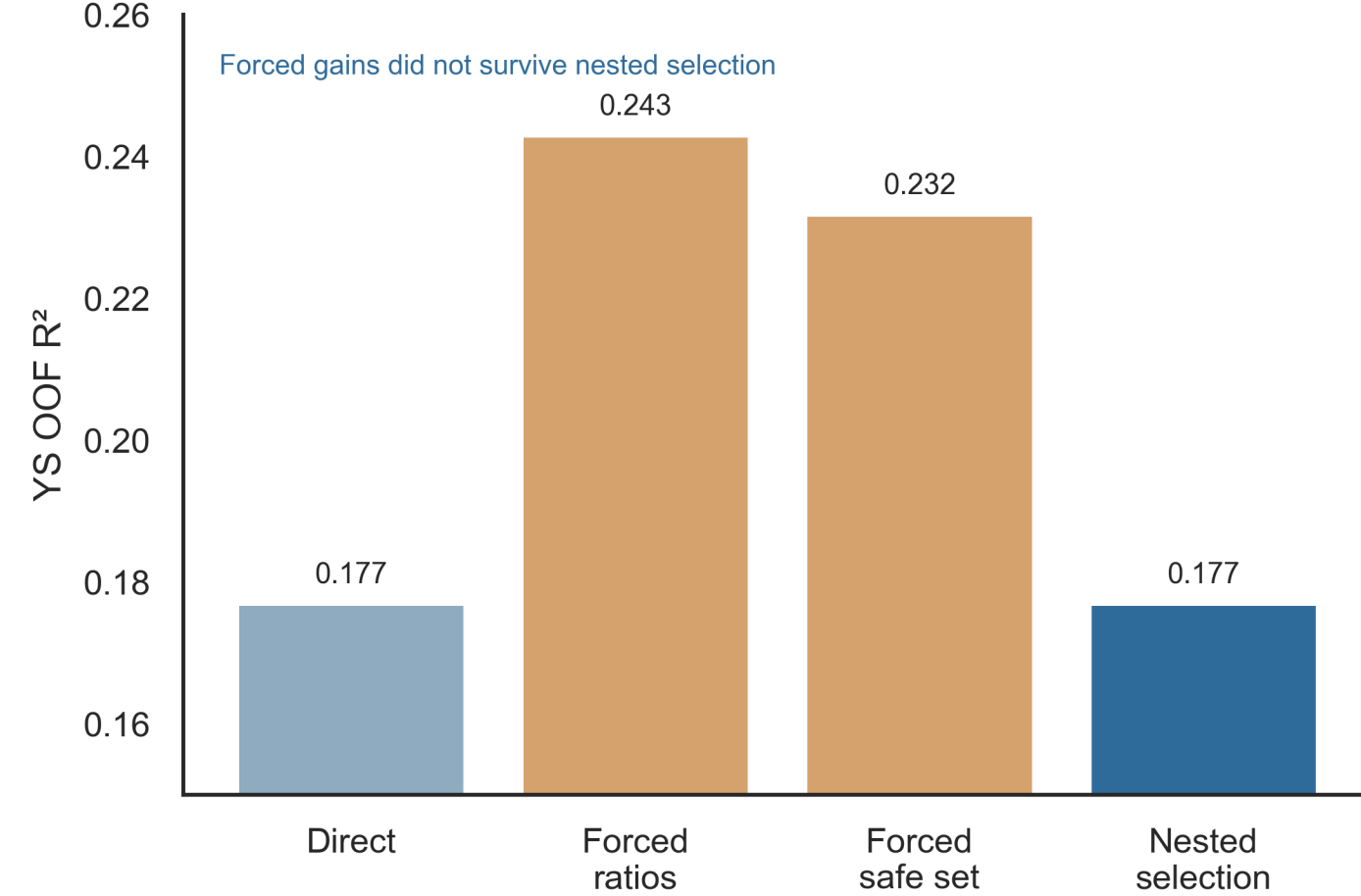
Derived-descriptor decision
