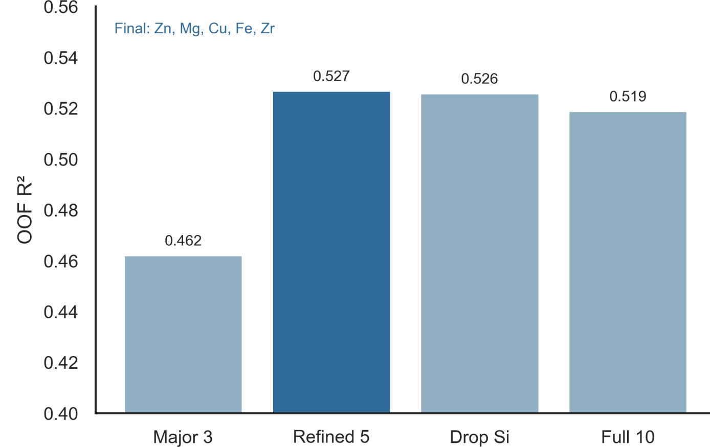
Sparse-feature decision
