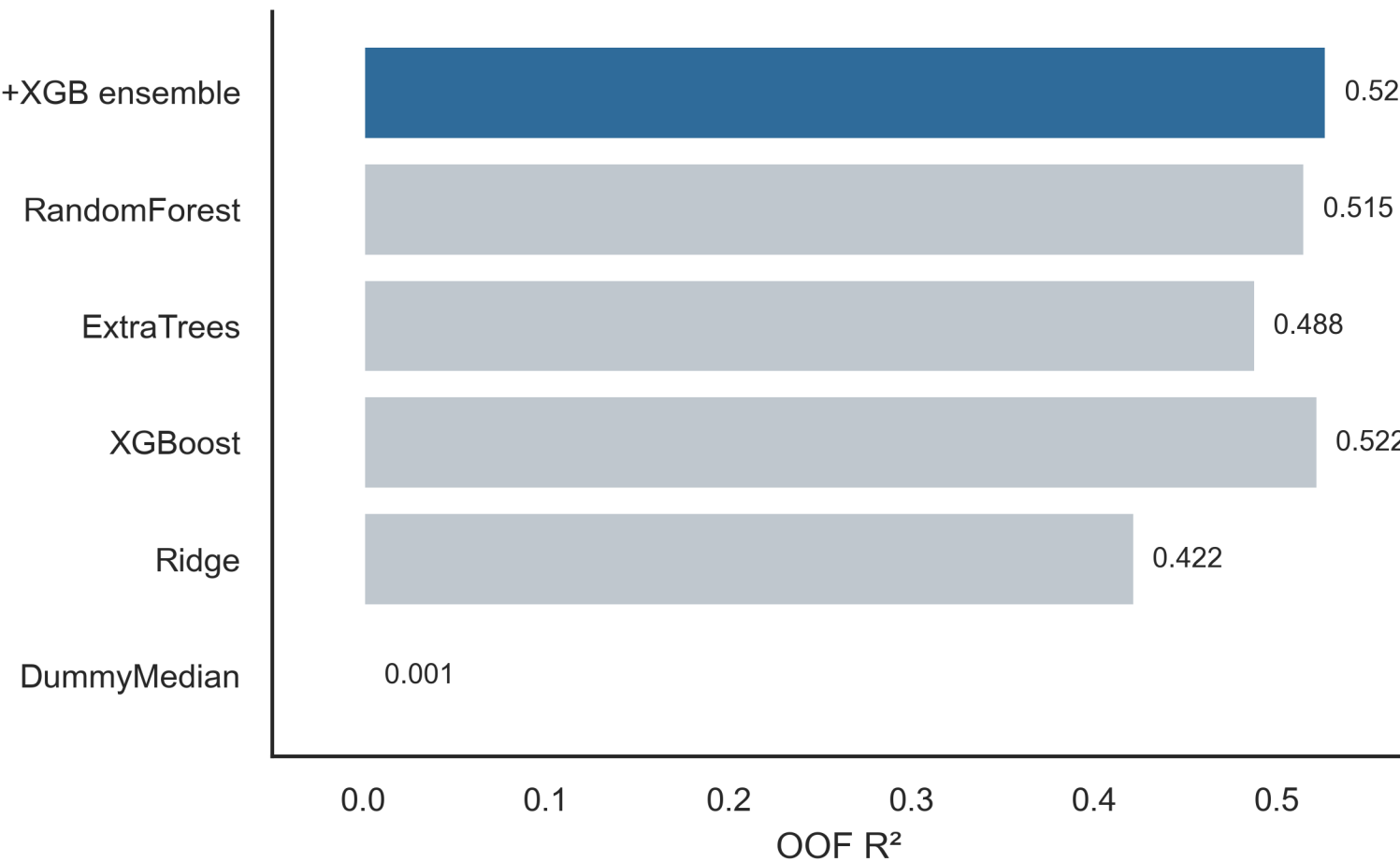
Model comparison under source-blocked CV
