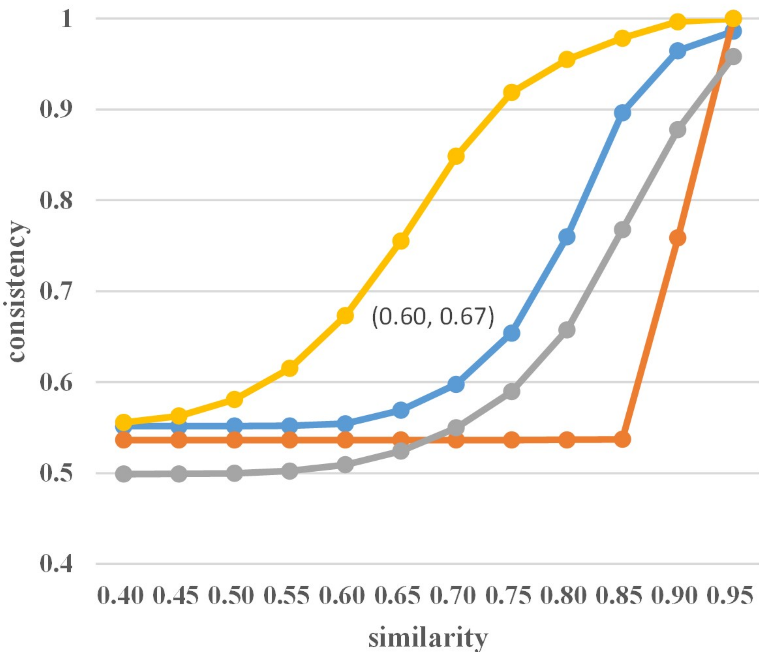
Cumulative Consistency
