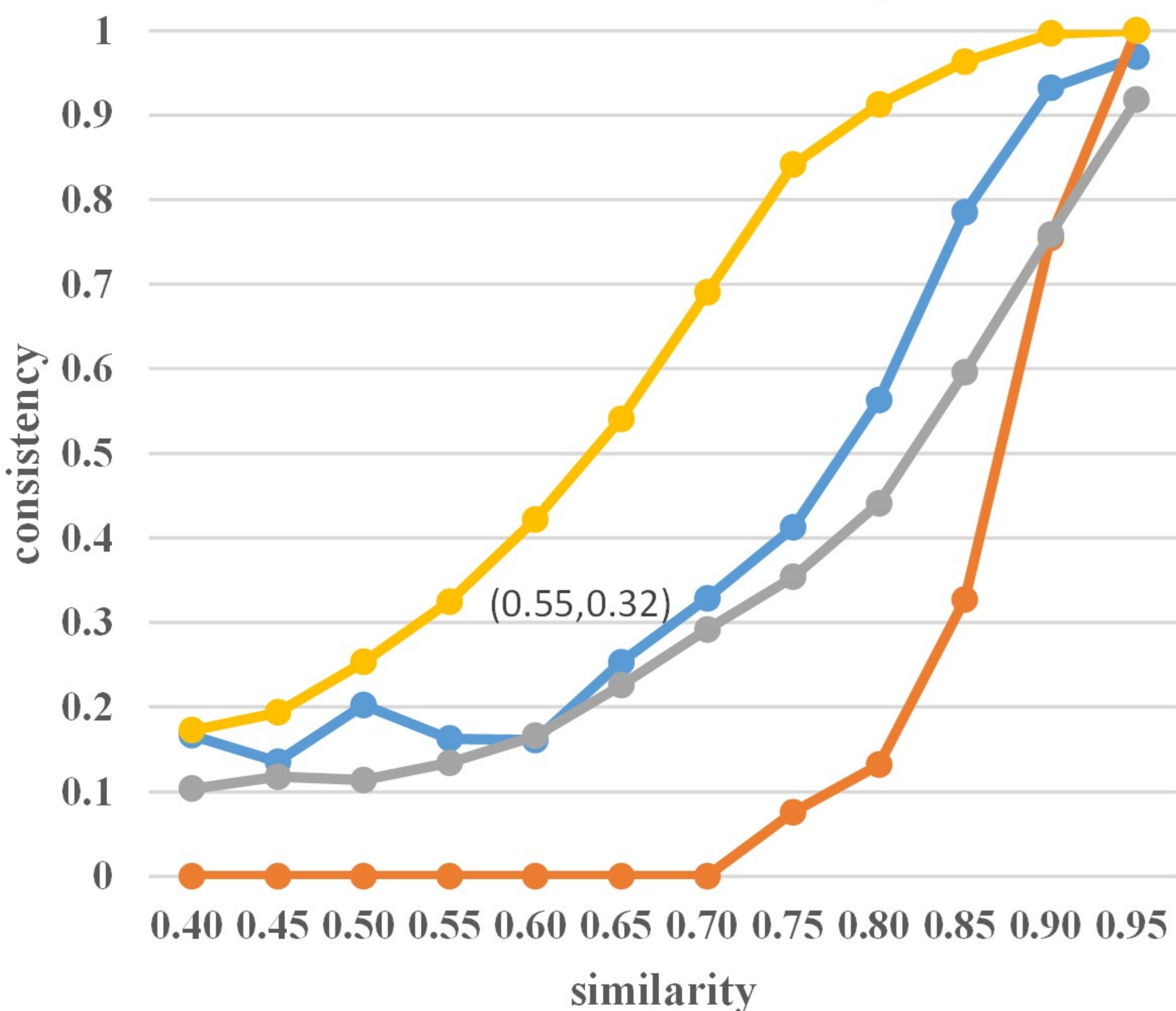
Bin-wise Consistency
